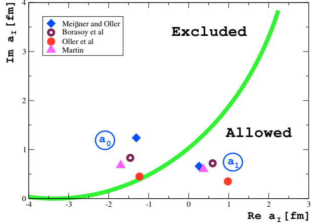
Fig. 1. Restrictions set by the DEAR data on the values of the scattering lengths a_0 and a_1 . For comparison, we give the scattering length calculations from different analyses: 1) Meißner and Oller [19], 2) Borasoy, Nißler and Weise, fit u [20], 3) Oller, Prades and Verbeni, fit A4 [21], 4) Martin [27].
