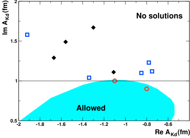
Fig. 2. The region in the (\text{Re } A_{Kd}, \text{Im } A_{Kd}) -plane where solutions for a_0 and a_1 exists. The cutoff parameter is \Lambda = 600 MeV. For comparison, we also show the results of calculations of the kaon-deuteron scattering length from table 3 (filled diamonds), the synthetic data from tables 5, 6 (squares) and our representative solutions from table 7 (circles).
