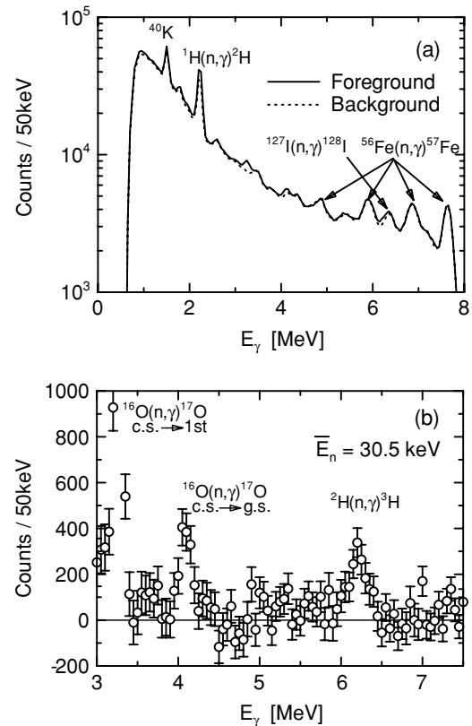
FIG. 3. \gamma -ray pulse height spectra from the ^2\text{H}(n, \gamma)^3\text{H} reaction. (a) Foreground and background spectra are respectively shown as the solid and dotted lines at 10 < E_n < 80 keV. (b) Background subtracted spectrum at 20 < E_n < 40 keV is shown.
