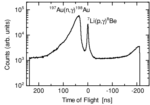
FIG. 2. TOF spectrum for ^{197}\text{Au} taken by the NaI(Tl) detector at E_n = 531 keV. The peak at 0 ns is from the ^7\text{Li}(p, \gamma)^8\text{Be} reaction and the broad peak is due to the \gamma ray from the keV neutron capture reaction by ^{197}\text{Au} .
