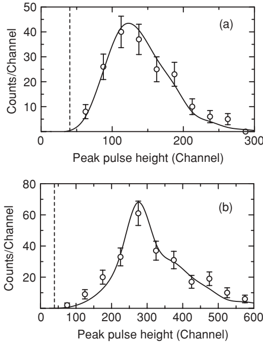
FIG. 6. Total pulse height spectrum from the {}^3\text{He}(\gamma, p)\text{D} reaction at E_{\gamma}^{\text{max}} = 16.5 MeV (a) and 10.5 MeV (b), respectively. The solid curves are the spectra calculated by a Monte Carlo method.
