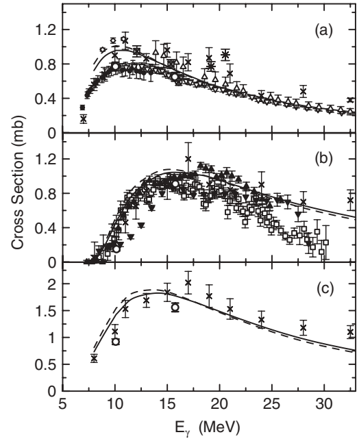
FIG. 12. ^3\text{He} photodisintegration cross section: (a) ^3\text{He}(\gamma, p)\text{D} , (b) ^3\text{He}(\gamma, pp)\text{n} , and (c) total photoabsorption. Present (open circles), Ref. [9] (crosses), Ref. [10] (filled downward triangles), Ref. [11] (filled circles), Ref. [12] (crossed squares), Ref. [13] (open upward triangles), Ref. [14] (asterisks), Ref. [15] (open downward triangles), Ref. [16] (crossed circles), Ref. [17] (open squares), Ref. [18] (diamonds), Ref. [19] (filled upward triangles). The solid curves and the dashed ones indicate the calculated cross sections using the inter-nucleon potentials of the AV18+Urbana IX and the AV18 alone, respectively.
