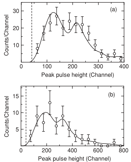
FIG. 8. Total pulse height spectrum from the {}^3\text{He}(\gamma, pp)n reaction at E_{\gamma}^{\text{max}} = 16.5 MeV (a) and 10.5 MeV (b), respectively. The solid curves are the spectra calculated by a Monte Carlo method.
