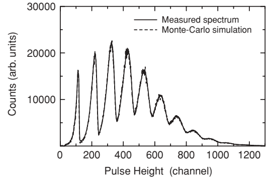
FIG. 10. Typical \gamma -ray pulse height spectrum measured at E_{\gamma}^{\text{max}} = 10.5 MeV with a BGO detector. The average \gamma -ray yield per pulse, M , was determined to be 4.48 by fitting the spectrum.
