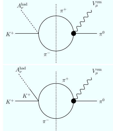
Fig. 3. \mathcal{O}(p^6) diagrams with cuts in the s -channel that contribute to the \text{Im}\{A_i\} . The big filled dots denote vertices from the Wess–Zumino–Witten Lagrangian. The second diagram with the kaon pole contributes to A_3 only.
