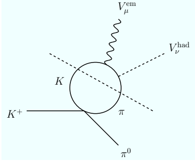
Fig. 1. Example of a \mathcal{O}(p^4) loop diagram with cuts for t \geq (M_K + M_\pi)^2 and W^2 \geq (M_K + M_\pi)^2 .
