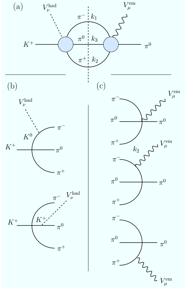
Fig. 4. Two-loop diagrams with three-pion cuts that contribute to the \text{Im}\{V_i\} .
