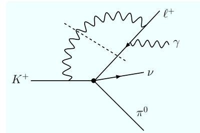
Fig. 8. Example of a photon loop diagram. For a complete listing of all Feynman diagrams that contribute to the imaginary parts via electromagnetic final-state interactions, see Fig. 5 in Ref. [16].
