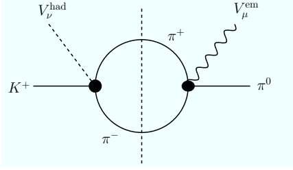
Fig. 5. Two-pion-cut diagram contributing to \text{Im}\{V_i\} at \mathcal{O}(p^8) .
