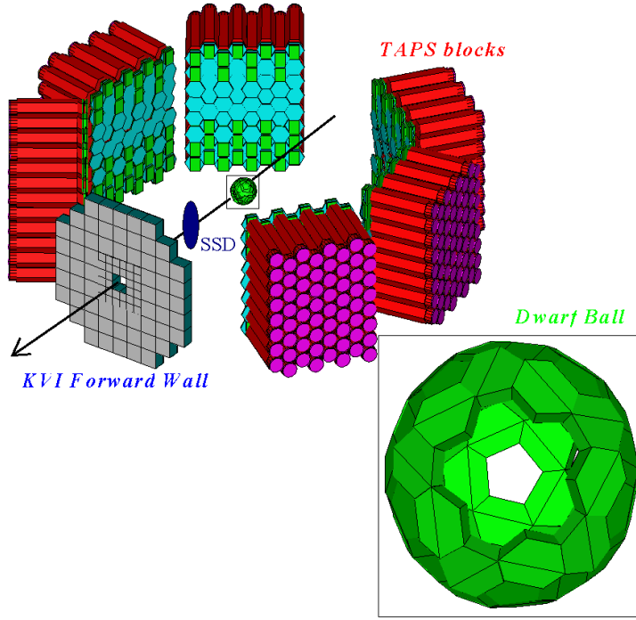
Fig. 1. General layout of the experimental setup used to study the reaction ^{129}\text{Xe} + ^{\text{nat}}\text{Sn} at 50A MeV at GANIL. The detector system consists of the Silicon Strip Detector (SSD), the Washington University Dwarf Ball (DB), the TAPS electromagnetic calorimeter and the KVI Forward Wall (FW).
