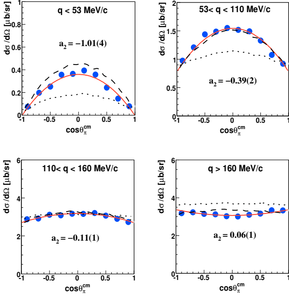
Fig. 11. Pion angular distributions (overall cm system) for 4 different q -ranges as indicated for the pp \rightarrow pp\pi^0 reaction. Data from this work are shown by full circles, the fit to the data with eq. 2 by solid lines. For the explanation of dashed and dotted lines see caption of Fig. 6.
