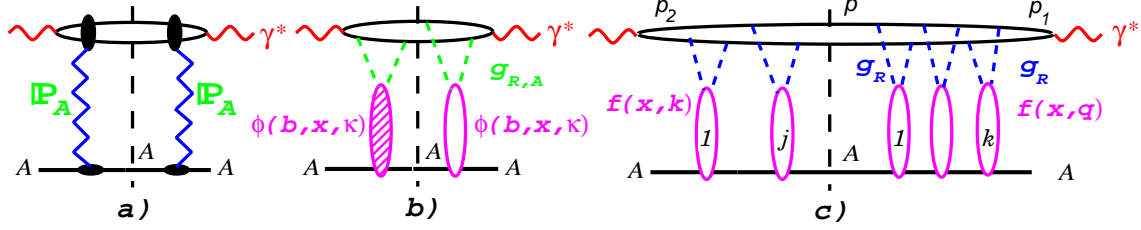
FIG. 6: (a) The diffractional unitarity cut with the ground state of the target nucleus in the intermediate state, (b) one of the 16 diagrams for diffractional unitarity cut in terms of couplings of coherent nuclear gluons g_{R,A} to quarks and antiquarks, (c) the total coherent diffractional cross section in terms of the \gamma^*(j\mathbf{IP})(k\mathbf{IP})\gamma^* impact factor.
