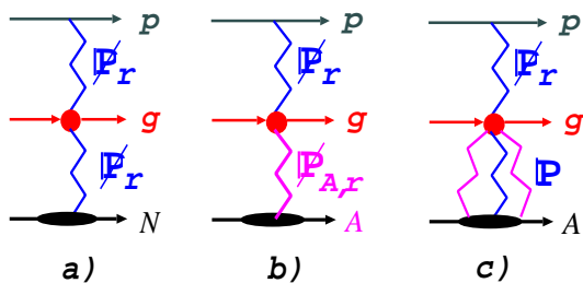
FIG. 16: The Kancheli-Mueller optical theorem for the mid-rapidity gluon spectrum: (a) for the free-nucleon target in terms of cut in-vacuum pomerons, (b) for the nuclear target with a cut nuclear pomeron on the nucleus side, (c) the anticipated multiple in-vacuum pomeron exchange on the nucleus side.
