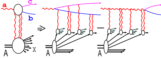
FIG. 2: Typical contribution to the excitation amplitude for aA \rightarrow bcX , with multiple color excitations of the nucleus. The amplitude receives contributions from processes that involve interactions with the nucleus after and before the virtual decay which interfere destructively. Notice a distinction between color-excitation (single-gluon, i.e., cut pomeron, exchange) and color-diagonal (elastic two-gluon, uncut pomeron, exchange) interactions between the target nucleus and the projectile and produced parton systems.
