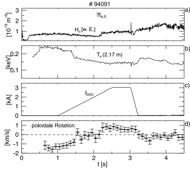
(a) DED 3/1 Konfiguration
