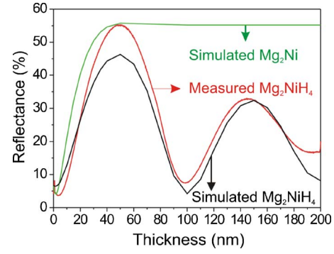
FIG. 5. (Color online) Reflectance at 1.95 eV vs deposited \text{Mg}_2\text{NiH}_4 thickness (red curve). The simulated reflectance of a \text{Mg}_2\text{NiH}_4 thin film (black curve) and of a \text{Mg}_2\text{Ni} thin film (green curve) are also shown. The good agreement between the measured reflectance and simulated reflectance indicates that \text{Mg}_2\text{NiH}_4 is synthesized in situ .
