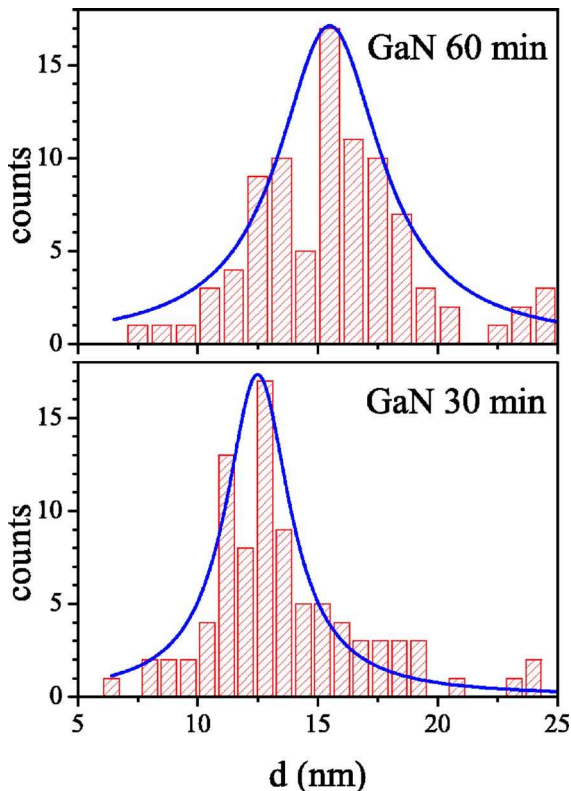
FIG. 2. (Color online) Histograms showing the distribution of the NW diameter in the nucleation growth regime for growth times of 30 and 60 min.
