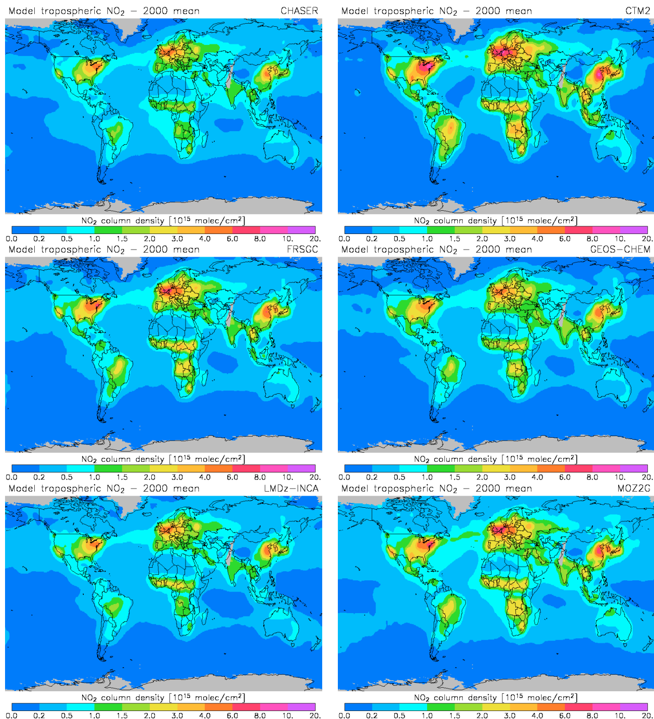
Fig. 2. Annual mean tropospheric NO 2 column density for the A-ensemble models. Data have been smoothed to a horizontal resolution of 5^\circ \times 5^\circ .
