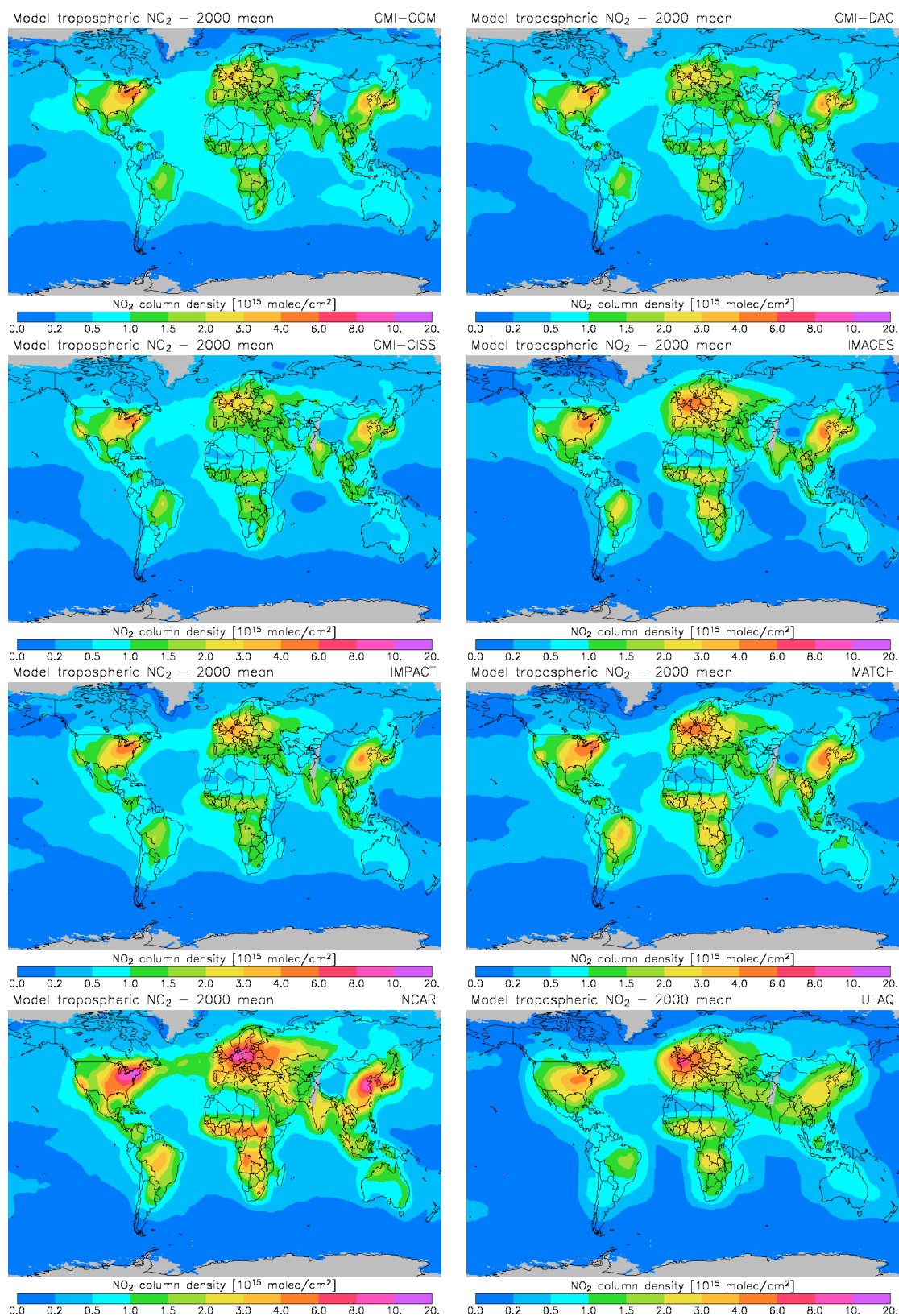
Fig. 3. Annual mean tropospheric NO 2 column density for the B-ensemble models. Data have been smoothed to a horizontal resolution of 5^\circ \times 5^\circ .
