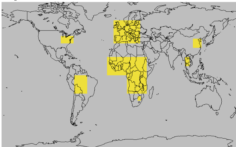
Fig. 9. Illustration of the various regions analyzed in this study: the eastern United States ( 90^{\circ}\text{W} – 71^{\circ}\text{W}\times 35^{\circ}\text{N} – 43^{\circ}\text{N} ), Europe ( 10^{\circ}\text{W} – 30^{\circ}\text{E}\times 35^{\circ}\text{N} – 60^{\circ}\text{N} ), eastern China ( 110^{\circ}\text{E} – 123^{\circ}\text{E}\times 30^{\circ}\text{N} – 40^{\circ}\text{N} ), South Africa ( 26^{\circ}\text{E} – 31^{\circ}\text{E}\times 28^{\circ}\text{S} – 23^{\circ}\text{S} ), Northern Africa ( 20^{\circ}\text{W} – 40^{\circ}\text{E}\times 0^{\circ}\text{N} – 20^{\circ}\text{N} ), Central Africa ( 10^{\circ}\text{E} – 40^{\circ}\text{E}\times 20^{\circ}\text{S} – 0^{\circ}\text{N} ), South America ( 70^{\circ}\text{W} – 50^{\circ}\text{W}\times 20^{\circ}\text{S} – 0^{\circ}\text{N} ), and Southeast Asia ( 98^{\circ}\text{E} – 105^{\circ}\text{E}\times 10^{\circ}\text{N} – 20^{\circ}\text{N} ).
