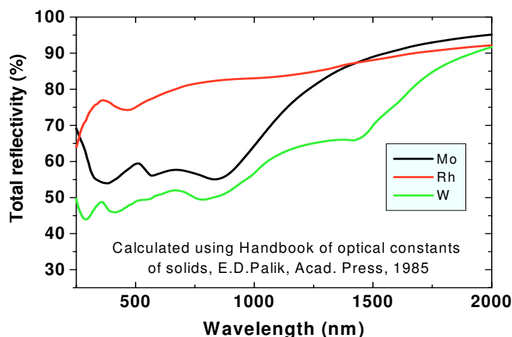
Figure 4 . The reflectivity as a function of a wavelength for molybdenum, tungsten and rhodium mirror materials.
