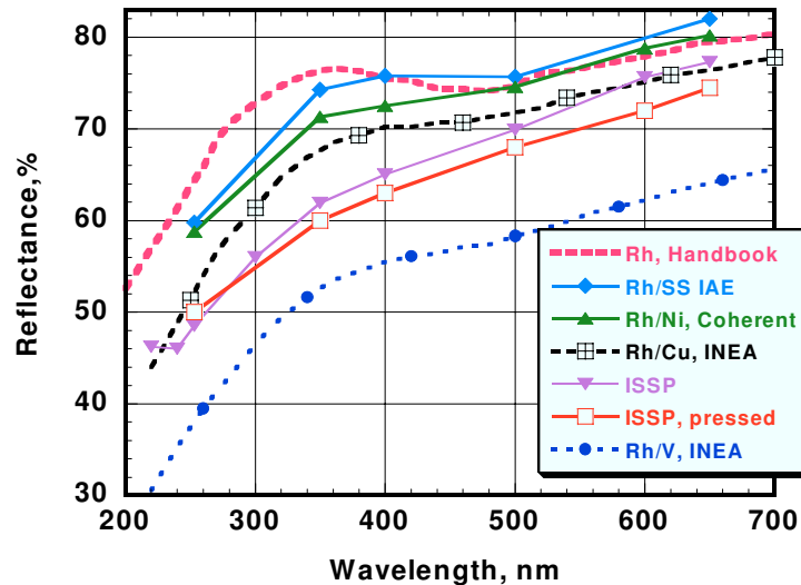
Figure 5. The dependence of a total reflectivity on a wavelength for Rh-coated mirrors from various producers [14].
