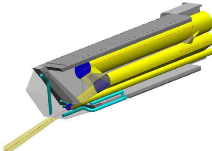
Figure 6. Scheme of core CXRS system for ITER with exchangeable diagnostic tubes
