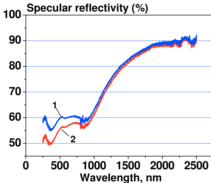
Figure 1: The specular reflectivity of molybdenum mirror after exposure in TEXTOR: 1) for SC Mo mirror 2) for PC Mo mirror;
