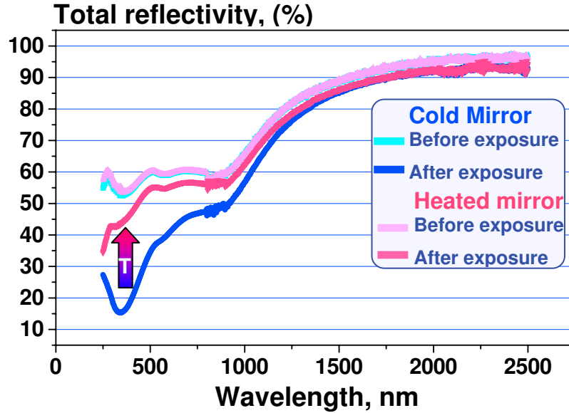
Figure 2: The evolution of the total reflectivity of molybdenum mirrors before and after exposures in DIII-D divertor. The data from [8] is used.
