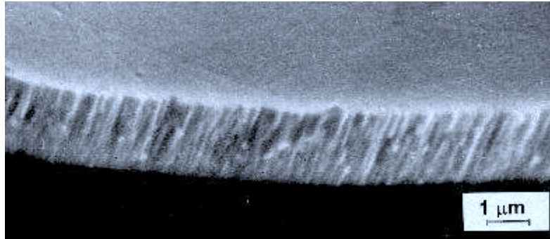
Figure3. Scanning Electron Microscope (SEM) image of a molybdenum film with a columnar structure [12].
