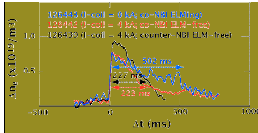
Fig. 6. Decay of pellet-induced density rises \Delta n_e in: (blue) ELMy H-mode with I-coil = 0 kA, (red) RMP-assisted ELM-free H-mode with 100% co-NBI, and (black) RMP-assisted ELM-free H-mode with 20% counter-NBI. The discharges have similar divertor recycling behavior.
