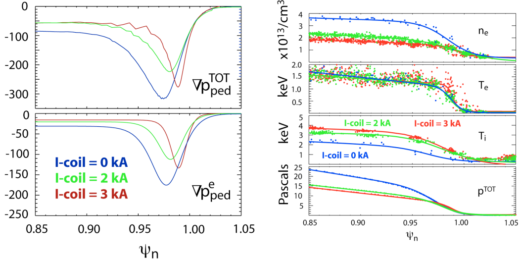
Fig. 4. (a) Pedestal total pressure gradient and (b) electron pressure gradient versus I-coil current in \delta=0.37 discharges. (c) Pedestal profiles of (top to bottom) n_e , T_e , T_i , and p^{\text{TOT}} versus I-coil current. Dots are data points; lines are hyperbolic tangent fits to the data. The profile for 0 kA (blue) is obtained by fitting Thomson and CER data in the last 20% of the ELM cycle. The 2 kA (yellow) and 3 kA (red) profiles are fits to all Thomson and CER data in 500 ms windows during ELM suppression.
