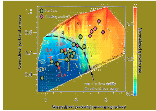
Fig. 5. Normalized P-B mode growth rates \gamma_N = \gamma/0.5\omega_e (where \gamma is the P-B growth rate and \omega_e is the electron diamagnetic drift frequency) for 6 ELMing cases (magenta diamonds) just before an ELM and 14 RMP-induced ELM-free (green ellipses) cases. \gamma_N is plotted as a function of the maximum value of the normalized pedestal pressure gradient \alpha = -(\mu_0/(2\pi)^2)\partial V/\partial\psi(V/2\pi^2R_0)\partial p/\partial\psi (where V is the plasma volume, p is the pressure, \psi is the poloidal magnetic flux and R_0 is the major radius of the plasma) and a characteristic pedestal current density j_N^{\text{ped}} , which is taken to be the peak value of the parallel current in the pedestal normalized by the average parallel current in the pedestal. Representative error bars, denoting one standard deviation, are shown on the data point at \alpha = 3.4 and j_N^{\text{ped}} = 0.53 . The color bar shows the value of \gamma_N for the color contours in the plot.
