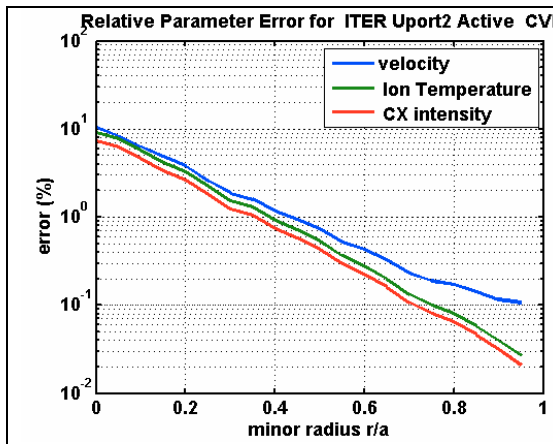
Fig.5a Error analysis: Ion temperature, toroidal rotation and ion density for C^{+6} . The concentration is 1% of electrons ( n_e(0)=10^{20}\text{ m}^{-3} ) and integration time is 100ms.
