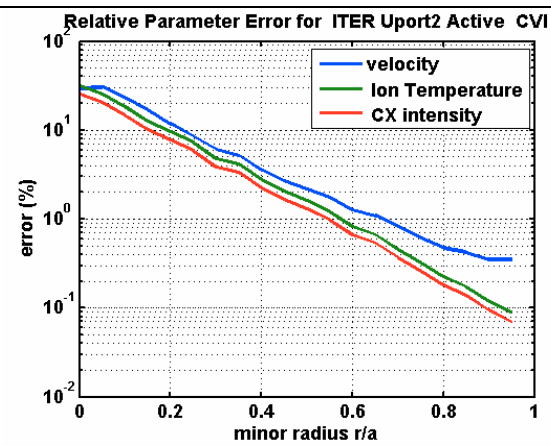
Fig.5b Error analysis: Ion temperature, toroidal rotation and ion density for C^{+6} . The concentration is 1% of electrons ( n_e(0)=10^{20}\text{ m}^{-3} ) and integration time is 10ms. Measurement requirements are satisfied for r/a > 0.2 .
