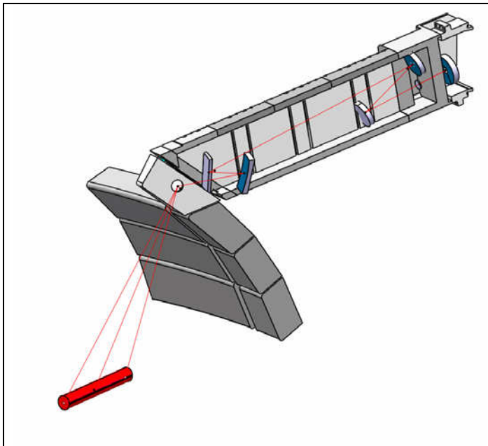
Fig.1 Schematic layout of Upper Port CXRS periscope with 100mm mono-crystal molybdenum ‘First-mirror’ in retracted position. A two-leg labyrinth system reduces the neutron level by several orders of magnitudes. The coupling to a transfer fibre bundle is achieved by using Cassegrain optics. The system has been optimised for light collection and, equally important, for high image quality in the case of periscope alignment when laser light produced fibre spots will be used with In-Vessel-Inspection-Cameras. The viewing area covers the entire DNB path between 0 < r/a < 1 .
