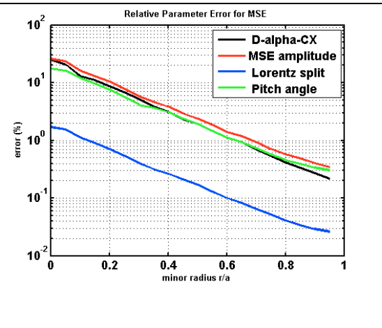
Fig.7 Parameter errors for Beam Emission and D-alpha CX amplitude
