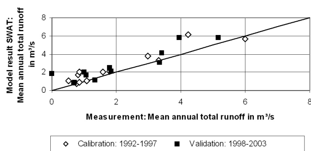
Fig. 5. Calibration and validation of the mean annual total runoff estimated by SWAT at gauged sub-catchments.
