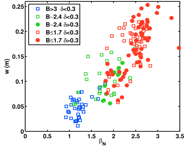
Figure 2. Island width versus normalised beta.
