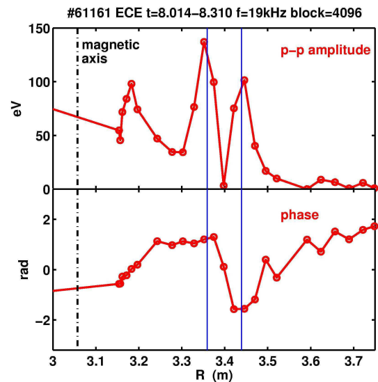
Figure 1. Amplitude and phase of T_e oscillations. Vertical blue lines mark island extremes.
