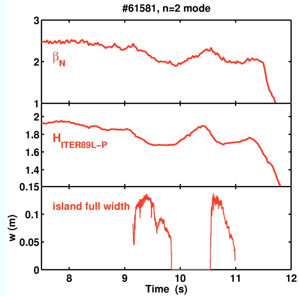
Figure 3. Time history of normalised beta, confinement and island width. Fishbones are present when w = 0 .
