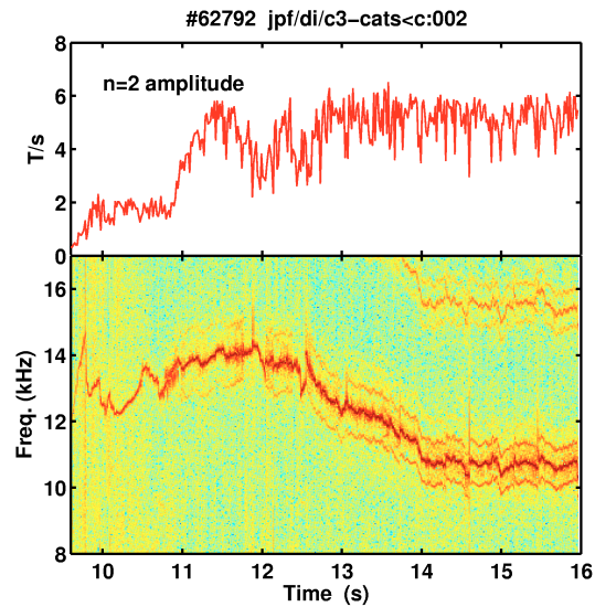
Figure 5. Time history of n=2 mode amplitude and spectrum showing the appearance of sidebands. An n=3 NTM (above 15 kHz) is also shown.
