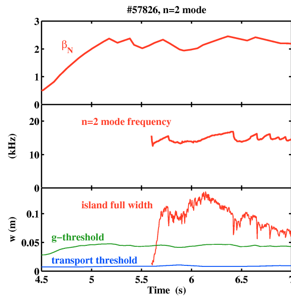
Figure 4. Time history of \beta_N , NTM frequency and island width showing a spontaneous NTM onset. Transport and ion polarisation (g) thresholds are shown.
