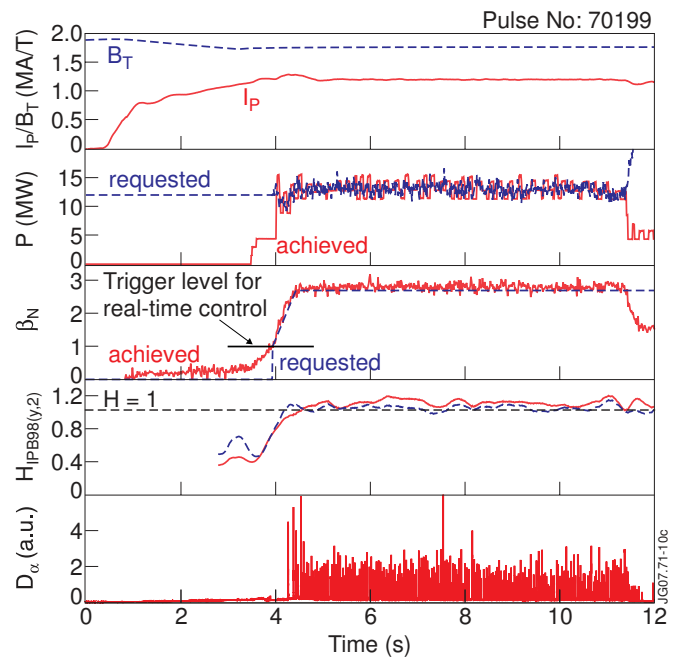
Figure 1. Time evolution of a typical high \beta_N pulse showing plasma current and magnetic field; requested and achieved NBI power; requested and achieved \beta_N ; H_{IPB98(y,2)} ; and D_\alpha , showing type I ELMs. H_{ITER98(y,2)} was evaluated using thermal stored energy from pressure profile integration (red) and W_{diamagnetic} - 1.5 \times W_{Jfast} using TRANSP NBI model [2] (blue).
