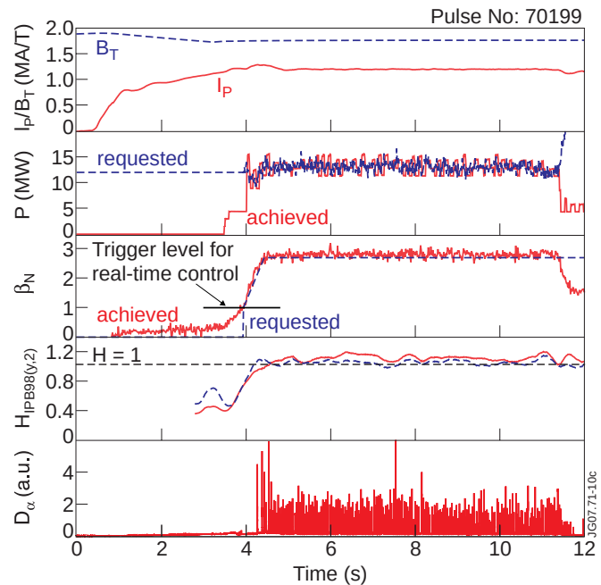
Figure 1. Time evolution of a typical high \beta_N pulse showing plasma current and magnetic field; requested and achieved NBI power; requested and achieved \beta_N ; H_{IPB98(y,2)} ; and D_\alpha , showing type I ELMs. H_{ITER98(y,2)} was evaluated using thermal stored energy from pressure profile integration (red) and W_{diamagnetic} - 1.5 \times W_{Jfast} using TRANSP NBI model [2] (blue).
