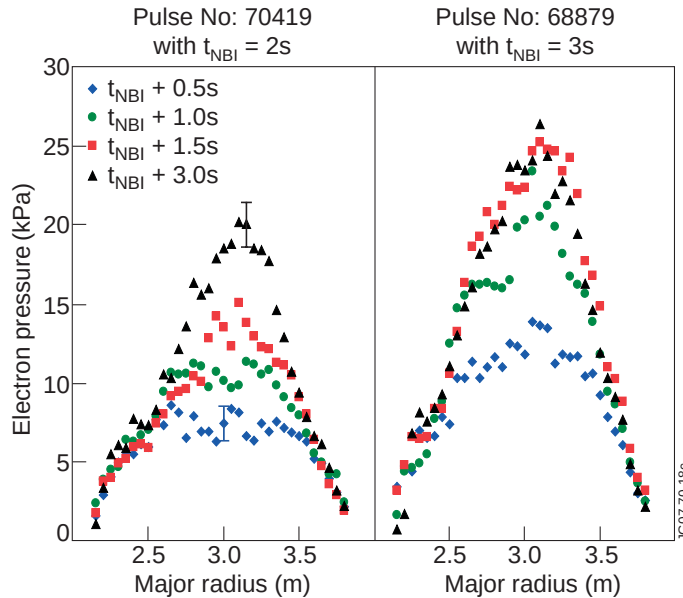
Figure 4. Electron pressure profiles measured using LIDAR showing the different evolution for pulses with different NBI start times. Each profile averaged over two points \pm 125 ms.
