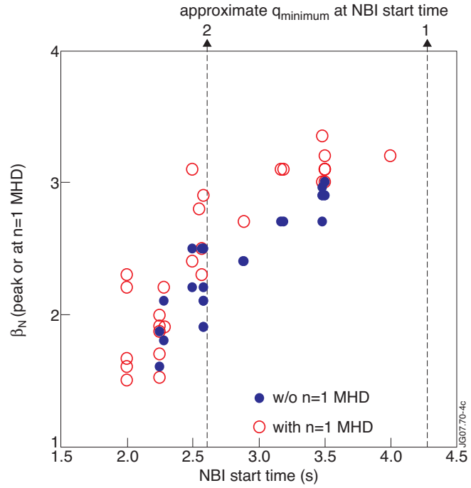
Figure 2. Maximum \beta_N (or the value at the start of performance limiting n=1 MHD activity) plotted against the start time of the main NBI heating.
