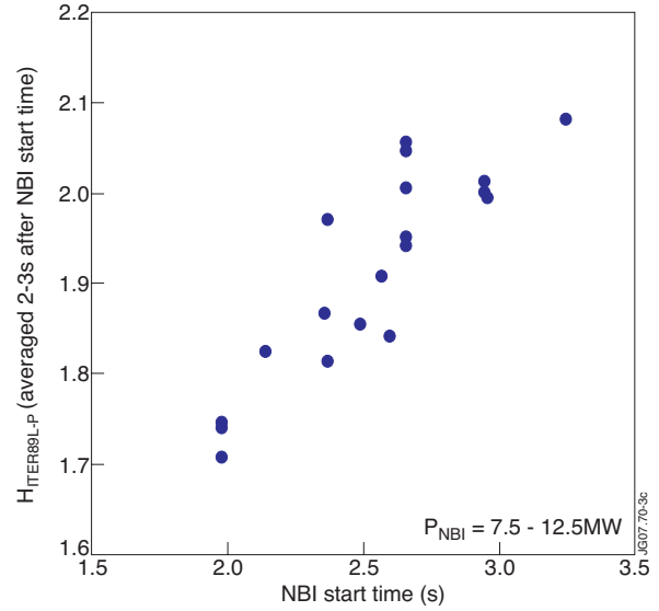
Figure 3. H_{ITER89L-P} averaged over the period 2-3s after the start of NBI plotted against NBI start time.
