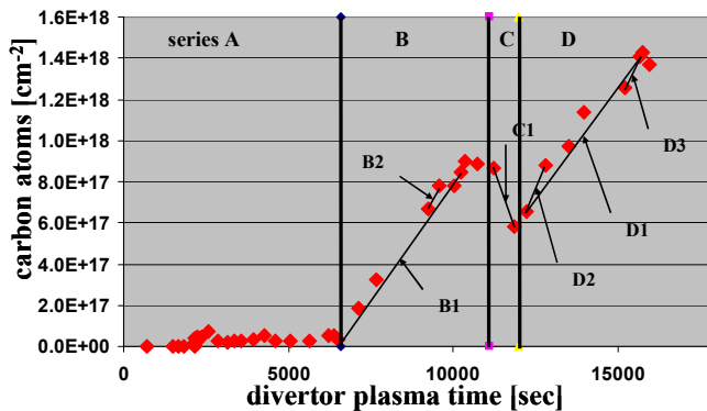
figure 2: erosion/deposition behaviour of a carbon layer in the private flux region of the MKII-HD divertor of JET
