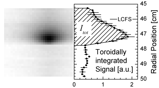
Fig. 4: typical CCD-camera image ( D_2 ) and toroidally integrated signal.
