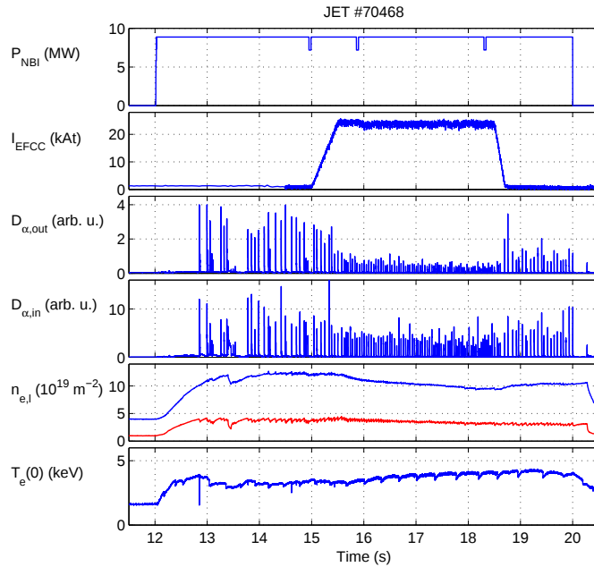
Figure 2: ELM mitigation with n = 2 field
