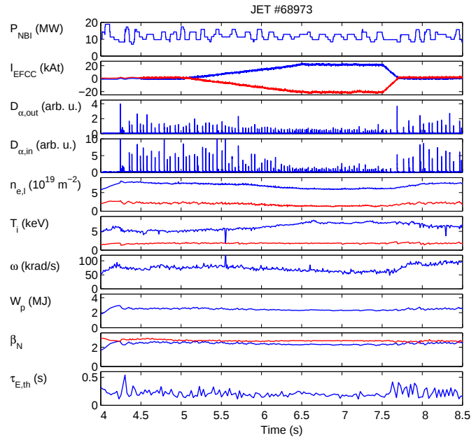
Figure 1: Overview of ELM control with n = 1 magnetic perturbation in a high beta discharge.
