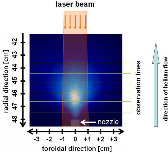
Figure 4: Beam emission at \lambda = 501.6 \text{ nm} ( 3^1\text{P}^o \rightarrow 2^1\text{S} ) recorded with a 2D-camera during the flat-top phase of a discharge with \bar{n}_e = 4 \times 10^{19} \text{ m}^{-3} . The path of the laser beam as well as the lines of sight are indicated.
