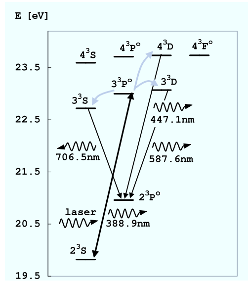
Figure 15: Pumping scheme for the measurements as shown in Figure 16. The grey arrows represent the collisional population transfer between the levels of the shell n = 3 - 4 .
