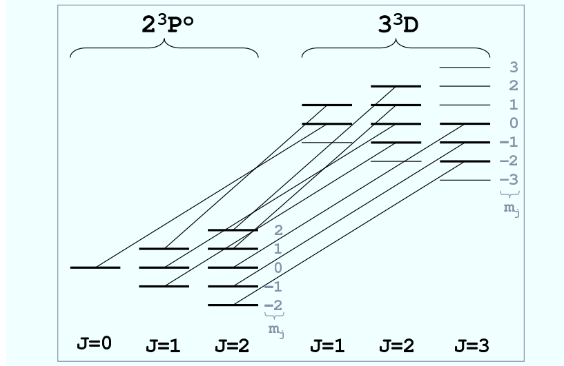
Figure 9: Part of the Grotrian diagram of Hel showing the Zeeman structure of the transition 3^3D \rightarrow 2^3P^0 at \lambda = 587.6 nm. Only those transitions are indicated which are listed in Table I, and correspond to the nine dominant \pi components of the line.
