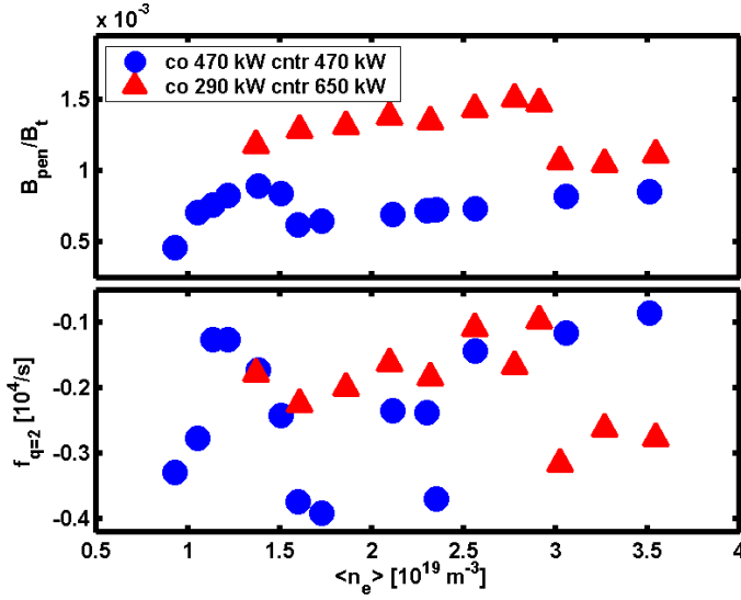
Figure 2: When the excitation threshold suddenly drops at the density of 1.5 \cdot 10^{19} \text{ m}^{-3} (circles) and at 3 \cdot 10^{19} \text{ m}^{-3} (triangles) the toroidal plasma rotation velocity at the q=2 surface also changes to further counter-rotation. No drop is found in the scan with only momentum input in co-direction.
