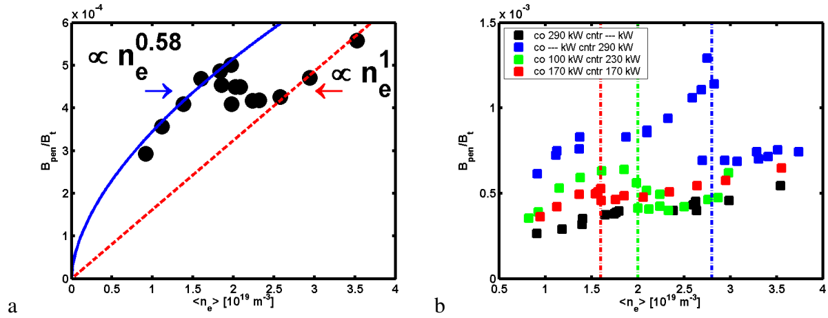
Figure 1: a) The calculated critical fraction B_{pen}/B_t which excites the 2/1 mode depends on the plasma density and shows a drop at the density of 2 \cdot 10^{19} \text{ m}^{-3} , in contrast to previously published scalings. b) The dashed lines indicate the sudden drop in the mode excitation threshold that is shifted to the left or right depending on the direction of the momentum input by the neutral beam injectors. It doesn't occur with only momentum input in co-current direction.
