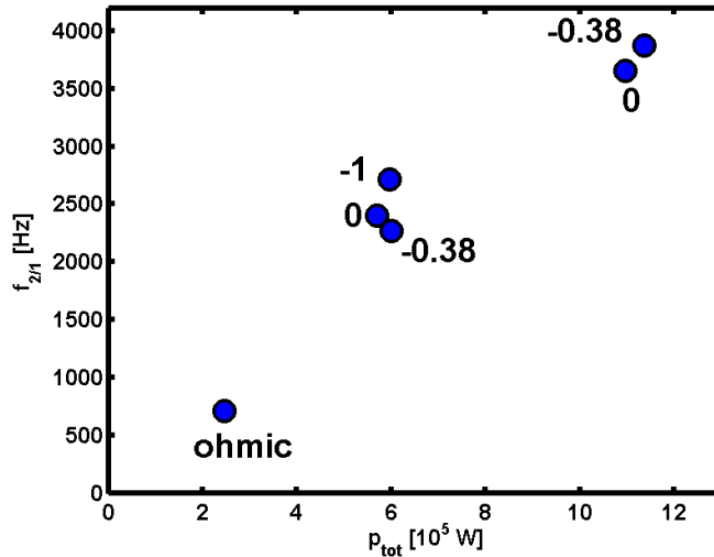
Figure 4: The frequency of the 2/1 mode before the sudden drop of the excitation threshold is plotted versus the total heating power (ohmic and neutral beam heating). The dependency is linear and independent of the neutral beam fraction \eta (indicated with the numbers)
