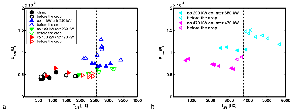
Figure 3: The dependency of the excitation threshold on the f_{2/1} -frequency a) with low neutral beam heating power and b) high neutral beam heating power. There is a critical frequency (marked as a dashed line) in each scan the frequencies accumulate at.
