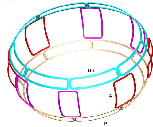
Figure 1: 3D view of active in-vessel coils
