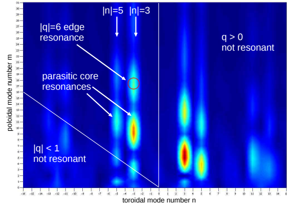
Figure 2: Mode number m, n spectrum perturbation (best fit to n = -3 at the q = -6 surface)
