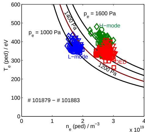
Figure 3: Edge operational diagram of the limiter H-mode at B_T = 1.9T
