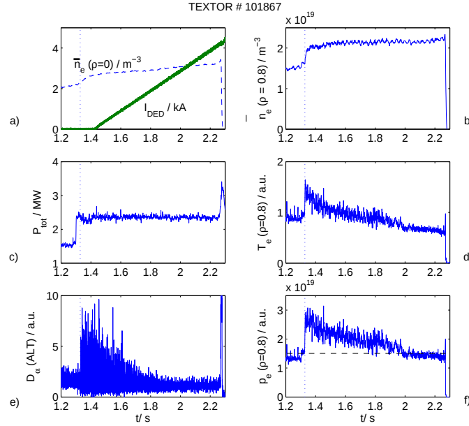
Figure 1: Response of the plasma edge properties to a slow ramp-up of the perturbation current in the 6/2 base mode configuration: a) line averaged central electron density (dashed) and perturbation current (solid line), b) line averaged electron density at \rho = 0.8 at the LFS, c) total input power, d) the electron temperature at the HFS at \rho = 0.8 , e) D_\alpha emission in front of the ALT limiter at the LFS, f) product of line averaged electron density at \rho = 0.8 at the LFS and the electron temperature at the HFS at \rho = 0.8 as a measure of the pedestal pressure
