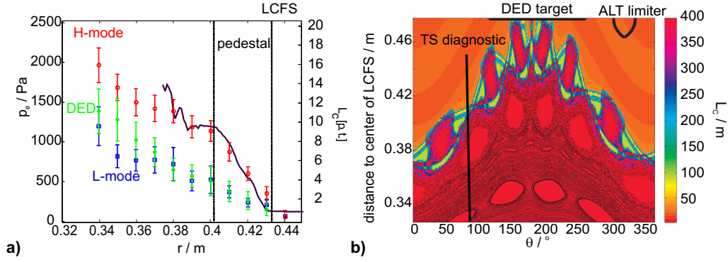
Figure 2: a) Edge electron pressure profiles for L-mode (blue squares, 102158), H-mode (red circles, 102161) and with DED (green diamonds, 102168) together with connection length to wall in poloidal turns, b) Laminar plot at toroidal section of TS diagnostic.
