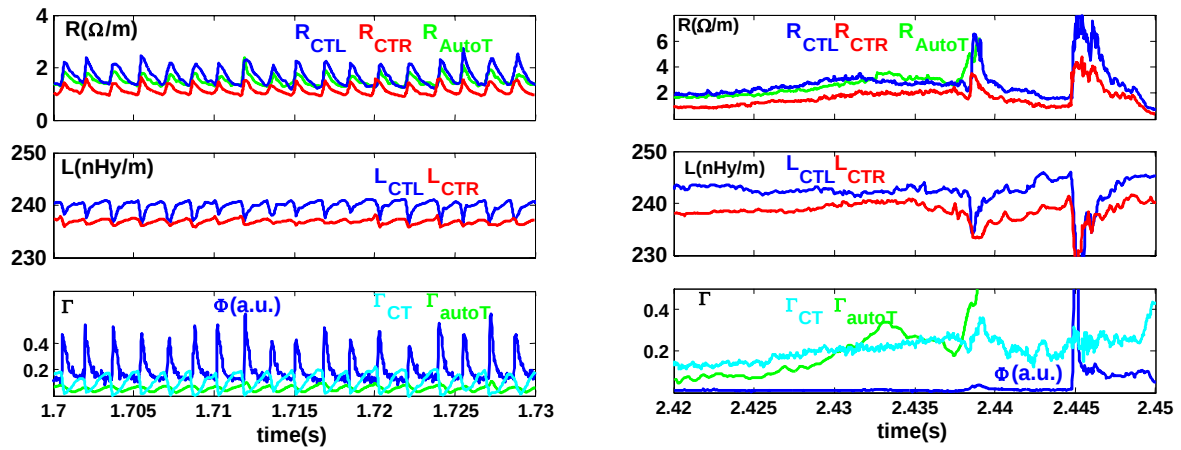
Figure 2 a) Antenna strap loading resistances and inductances (of the classically matched antenna: R_{autoT} , of the left and right straps of the CT antenna: R_{CTL} and R_{CTR} , L_{CTL} and L_{CTR} ), reflection coefficients (in the common branch of the classically matched antenna: \Gamma_{AutoT} , in the common branch of the CT: \Gamma_{CT} ) and recycling flux \Phi during ELMs. b) Idem but different time window.
