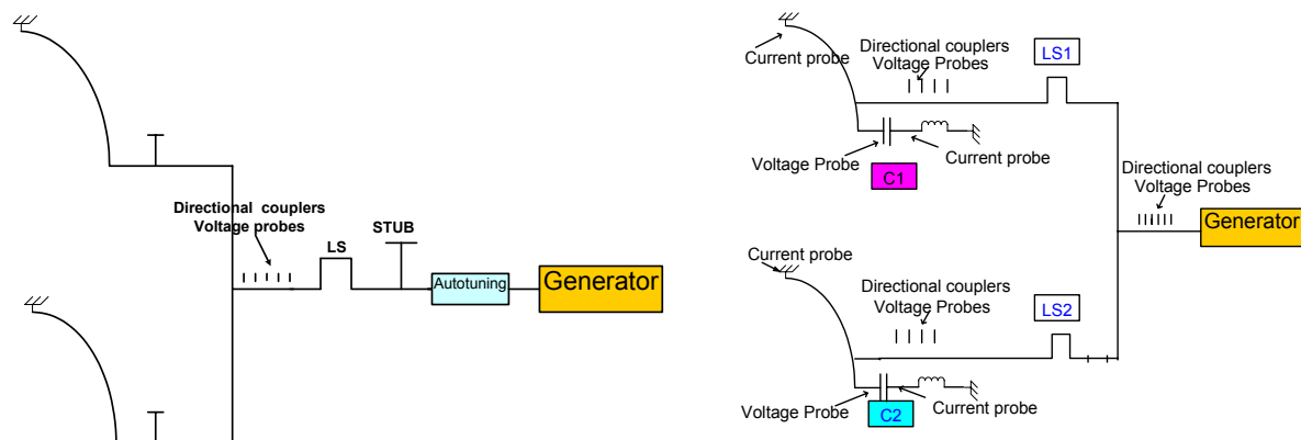
Figure 1 (a) Classically matched antenna (b) Conjugate-T antenna circuit and measurements.
