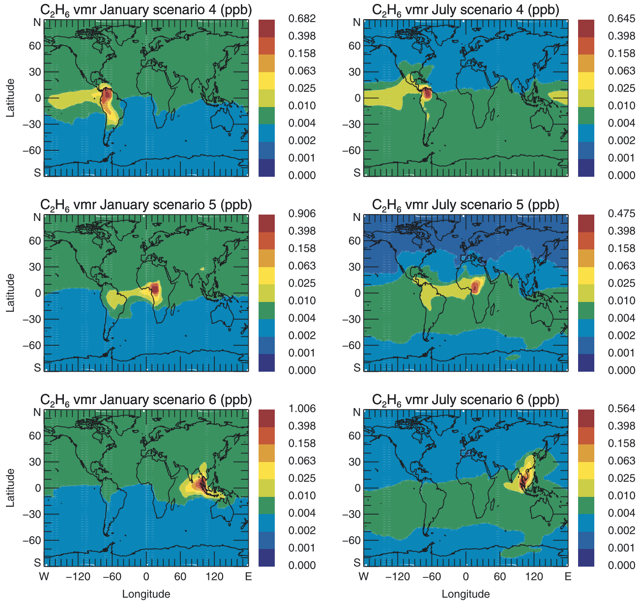
Figure 7. Modeled January and July \text{C}_2\text{H}_6 mixing ratios near the surface for emission scenarios 4–6 (lowest four levels, approximately lowest 700 m above ground).
