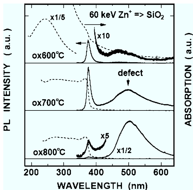
FIG. 3. Photoluminescence (solid lines) and optical absorption (dotted lines) spectra of \text{SiO}_2 samples implanted with \text{Zn}^+ ions of 60 keV to a fluence of 1.0 \times 10^{17} ions/ \text{cm}^2 , and annealed in oxygen gas for 1 h at 600, 700, and 800 °C, respectively. The spectra are shifted vertically for clarity and the vertical lines indicate the base lines. A part of the spectrum at 600 °C is also shown with magnification of ten times.
