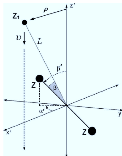
FIG. 3. Geometry of the Z_1 + e\text{ZZ} collision.
