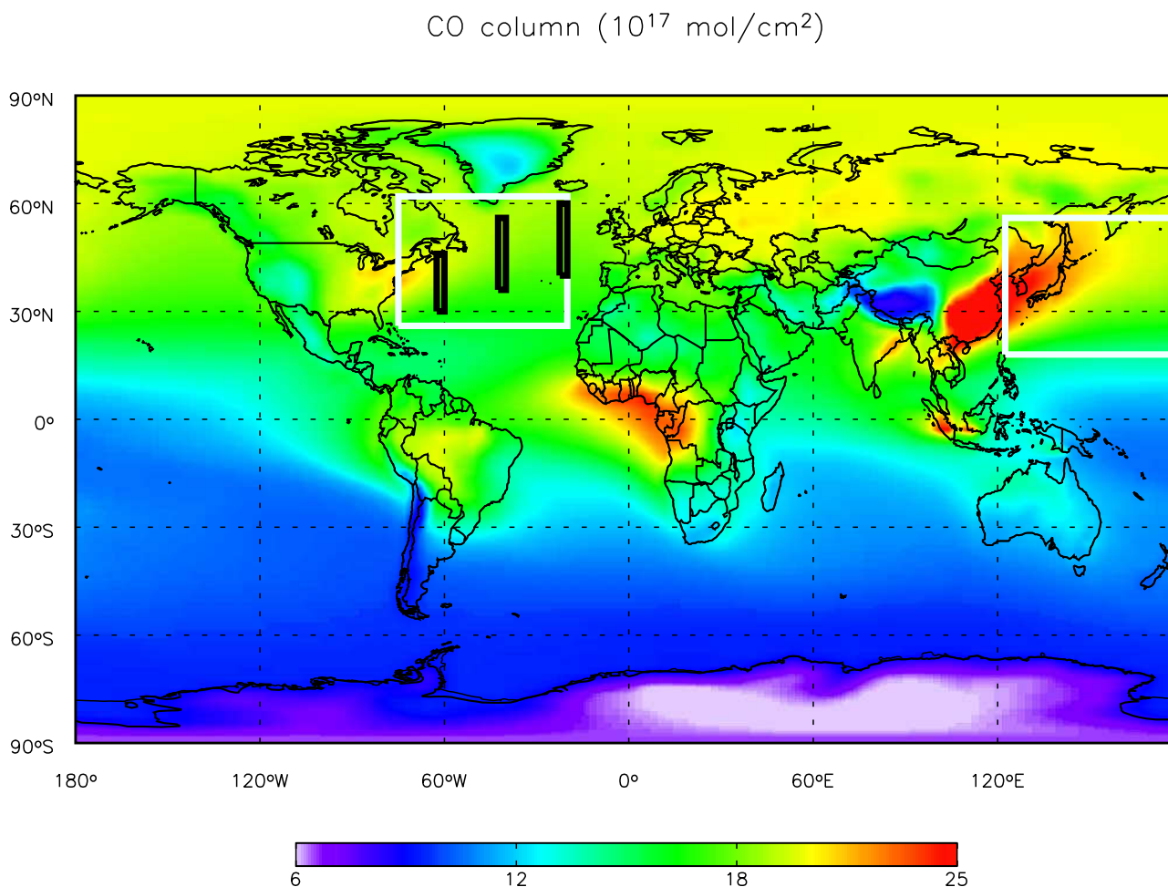
Figure 5. Geographical locations of the study regions described in this paper superimposed onto the annual mean GEOS-Chem CO column ( 10^{17} molecule/cm 2 ) integrated from the surface up to 180 mbar. North Atlantic region is 26–62°N, 75–20°W. Northwest Pacific region is 18–56°N, 122.5–177.5°E. The three black lines over the North Atlantic Ocean show the locations of the slices examined in section 4.
