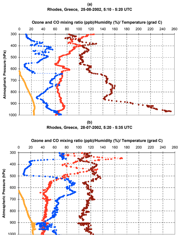
Fig. 7. Vertical profiles at Rhodes for a high ozone day (upper panel, a ) and a low ozone day (lower panel, b ), of CO (brown), ozone (red), relative humidity (blue) and temperature (orange).
