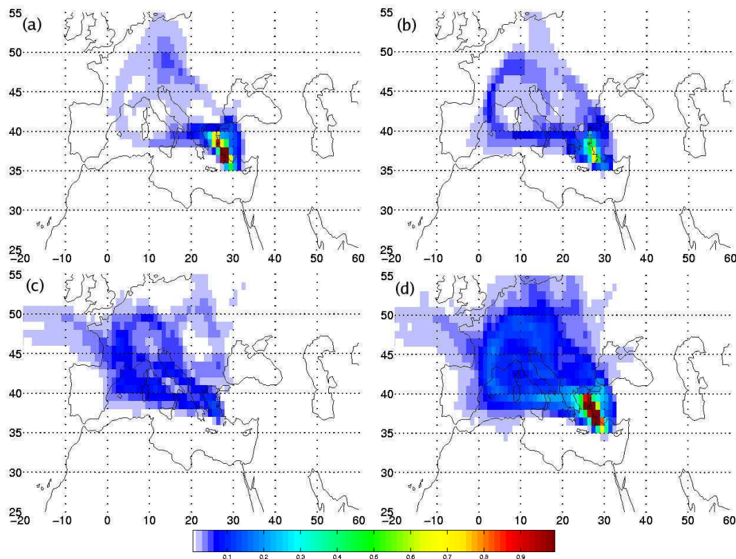
Fig. 5. Percentage contribution of geographical regions after 10-days FLEXPART backward simulation for the 4 high ozone cases and for the 0–2 km air parcels arriving at Rhodes. (a) for the 0–2 km layer, (b) for the 2–4 km layer, (c) for the >4 km layer and (d) for the total atmospheric column.
