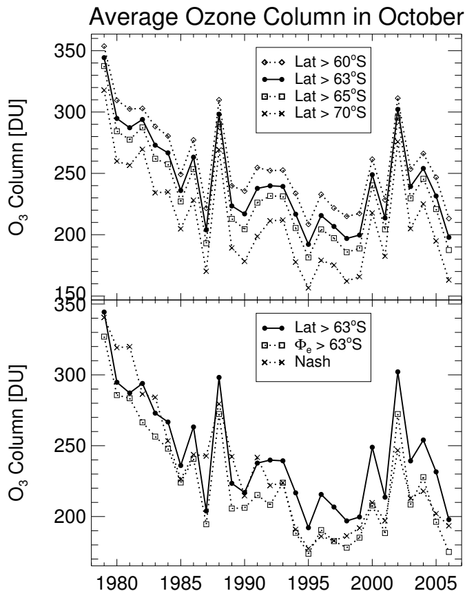
Fig. 2. Top panel: October mean Antarctic total column ozone averaged poleward of 60°S, 63°S, 65°S, and 70°S. Bottom panel: October mean Antarctic total column ozone averaged poleward of 63°S compared with calculations using the equivalent latitude \Phi_e = 63^\circ\text{S} and the Nash-criterion (applied on the 475 K potential temperature surface) as vortex edge definitions.
