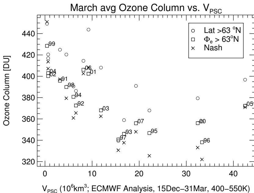
Fig. 10. The relation between V_{\text{PSC}} and the total column ozone in March averaged over the Arctic polar region. Circles show averages poleward of 63^\circ\text{N} , squares averages poleward of 63^\circ\text{N} equivalent latitude, and crosses averages poleward of the vortex edge defined by the maximum gradient in potential vorticity.
