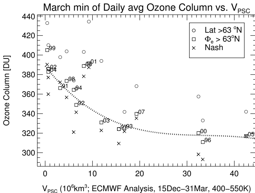
Fig. 11. The relation between V_{\text{PSC}} and the minimum of March daily average polar column ozone (symbols as in Fig. 10). The dotted line shows an empirical fit through the minimum ozone values for averages poleward of an equivalent latitude of 63^\circ\text{N} with the exception of the years 1999, 2001, and 2006 for which the final warming occurred before March. Not shown (and excluded from the fit) is the year 1995 because of poor data quality; only 3% of the data points poleward of 63^\circ equivalent latitude are valid. The polynomial describing the fit is given by M = 388.6 - 6.10 \cdot V + 0.178 \cdot V^2 - 0.00176 \cdot V^3 , where V is V_{\text{PSC}} in 10^6 \text{ km}^3 and M is the minimum of March daily average polar column ozone in Dobson units (this relation being valid for V_{\text{PSC}} < 42.5 ).
