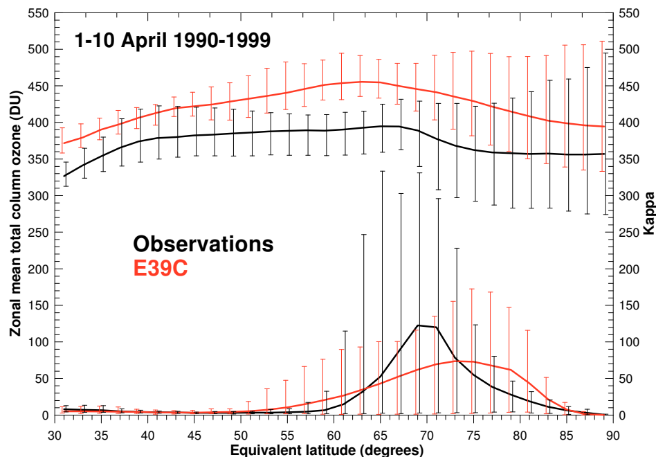
Fig. 7. Equivalent latitude (on the 550 K surface) zonal mean total column ozone (top two curves plotted against the left ordinate), and the strength of the barrier to meridional transport \kappa , (bottom two curves plotted against the right ordinate) for the northern hemisphere averaged over the years 1990–1999 and 1–10 April. Observations are shown in black and model results (from the transient run of E39/C, Dameris et al., 2005 ) in red. The vertical bars show the extremes (maximum and minimum values over the period).
