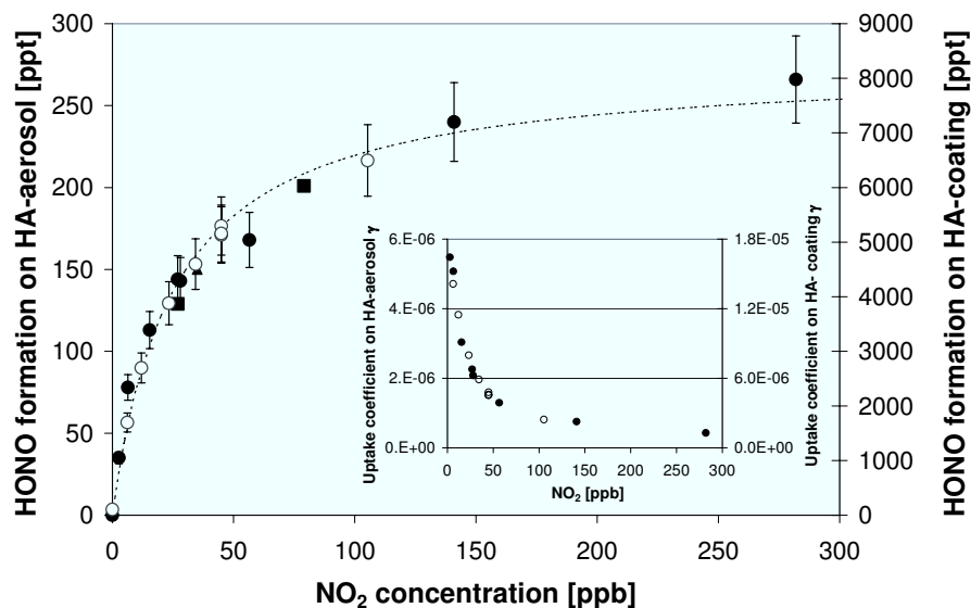
Fig. 5. Dependence of the HONO-formation on humic acid (HA) aerosols on the \text{NO}_2 -concentration (filled symbols). The experimental conditions are as follows: reaction time 2.8 min, aerosol surface concentration 0.151 \pm 0.006 \text{ m}^2 \text{ m}^{-3} , relative humidity 26%, actinic flux 1.0 \times 10^{17} \text{ photons cm}^{-2} \text{ s}^{-1} in the 400–750 nm range. The filled squares and the filled triangle are from the experiments in Fig. 3 (■) and in Fig. 4 (▲) under most similar, but not completely identical conditions. The thin dashed line represents a model description of the results (Eq. 4). The empty circles (○, right scale) show the dependence of the HONO-formation on the \text{NO}_2 -concentration as observed on humic acid (HA) coatings at 21% relative humidity. The inset shows the dependence of the reactive uptake coefficient of \text{NO}_2 on humic acid (HA) aerosol (●, left scale) and humic acid (HA) coatings (○, right scale) as a function of the \text{NO}_2 -concentration.
