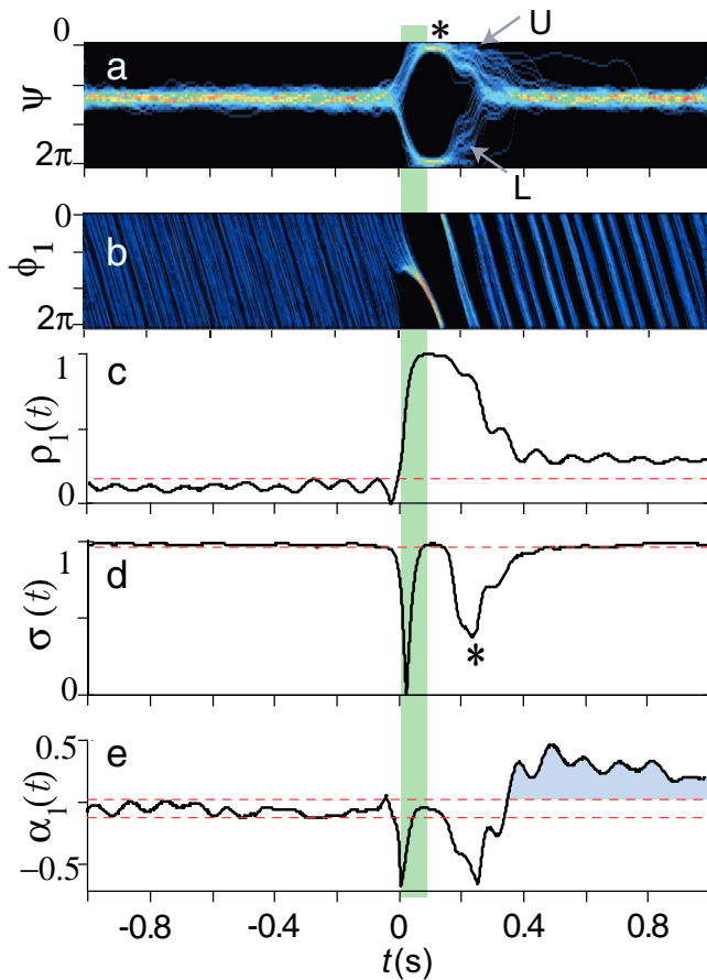
FIG. 6. (Color) Transient phase dynamics after simultaneous 75 ms inhibitory stimulation of a network of two electroreceptor bursters, each with inhibitory feedback and excitatory mutual coupling, as in Fig. 4. The stimuli, at random times, are indicated by a vertical bar at t=0 across panels (a)–(e). (a) Time-dependent probability density of the phase difference of the two bursters. Low values are indicated by blue, high values by red, and zero by black. Arrows show upper ( U ) and lower ( L ) branches of trial trajectories (see text). (b) Time-dependent probability density of the phase of burster #1, relative to the onsets of stimuli. Note double-peaked structures in the poststimulus domain, denoted as blue bands separated by narrow black stripes. (c) Time course of resetting index for burster #1. The dashed line indicates the significance level at the 99th percentile of the prestimulus ( t < 0 ) distribution. (d) Time course of synchronization index. (e) Time course of clustering index for burster #1. The shaded area indicates a statistically significant epoch of clustering.
