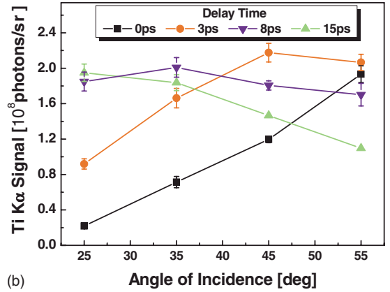
FIG. 8. (Color online) K\alpha emission per pulse as a function of the angle of incidence at fixed prepulse delay. a) Cu at \Delta t=0, 4, 7 , and 15 ps. b) Ti at similar delay times.
