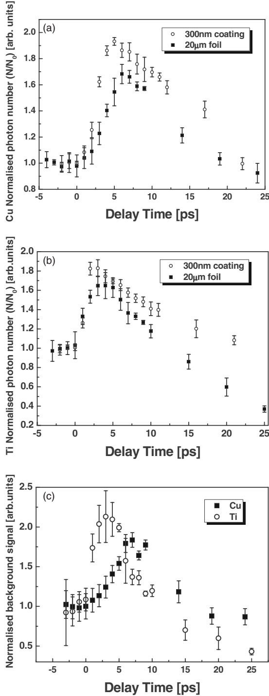
FIG. 5. Normalized K\alpha emissions per pulse as a function of main pulse delay at fixed angle of incidence of 45^\circ on different target thickness. (a) Cu-Target, N_0=5.2 \times 10^8 photons/sr and 8.2 \times 10^7 photons/sr for d=20 \mu\text{m} and 300 nm, respectively. (b) Ti-Target, N_0=1.4 \times 10^9 photons/sr and 1.2 \times 10^8 photons/sr for d=20 \mu\text{m} and 300 nm, respectively. (c) Hard x-ray background signal as a function of main pulse delay on 20 \mu\text{m} targets.
