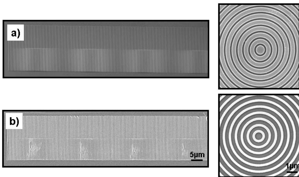
Figure A.10: SEM images (10 kV) of master and stamps with Moire patterns according to [Moers 2006]
