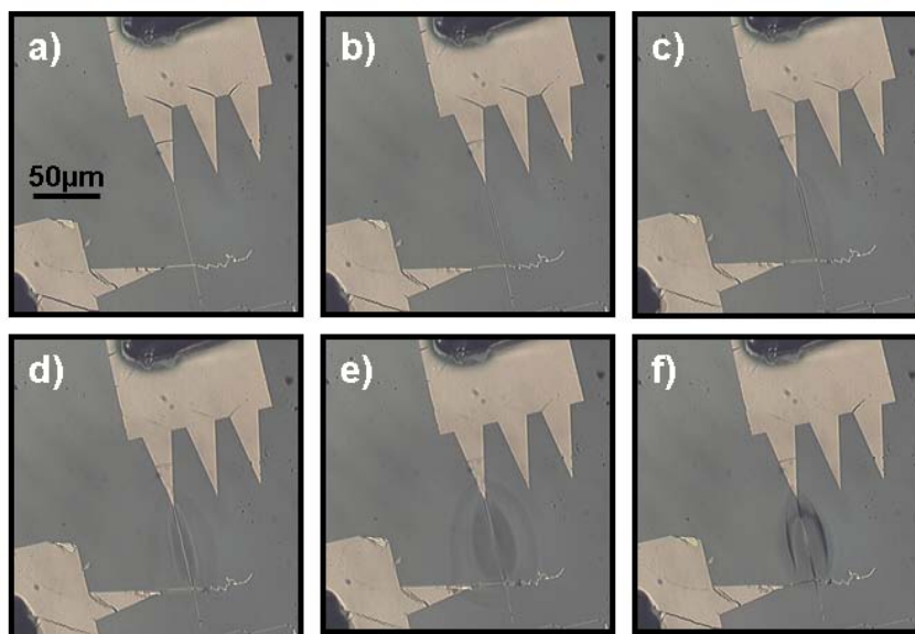
Figure A.20: Microscope images showing the melting of Affinity VP
