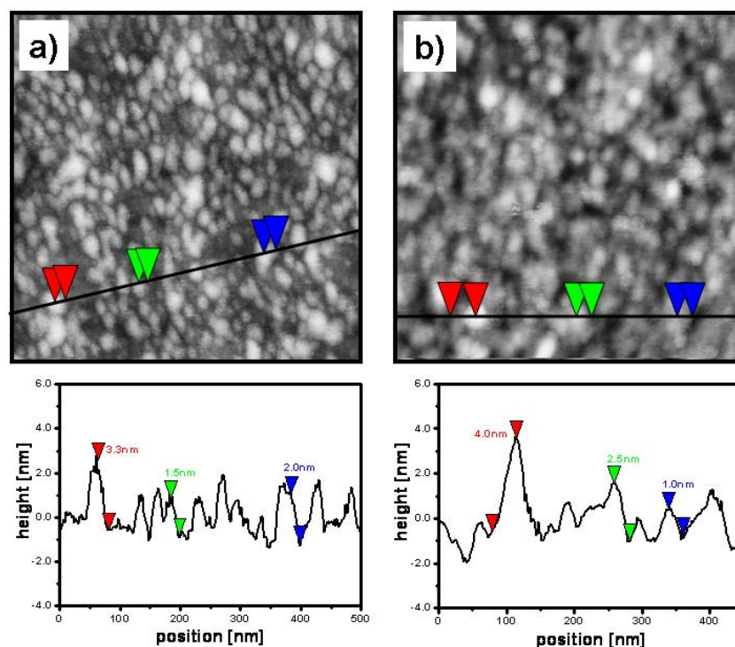
Figure 4.64: Tapping mode AFM images of gold surfaces
