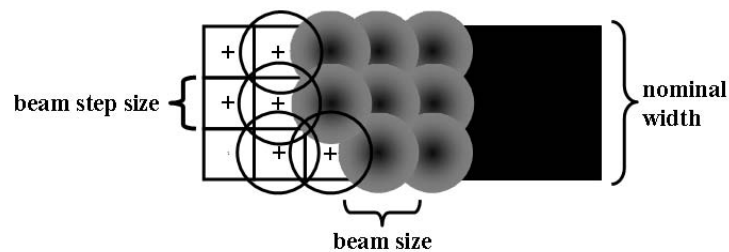
Figure 2.8: Schematic of the Gaussian Vector Scanning
