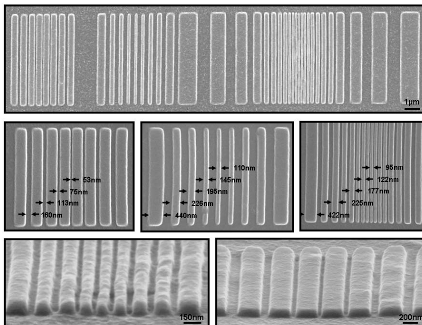
Figure 4.23: SEM (10 kV) images of a Surlyn stamp
