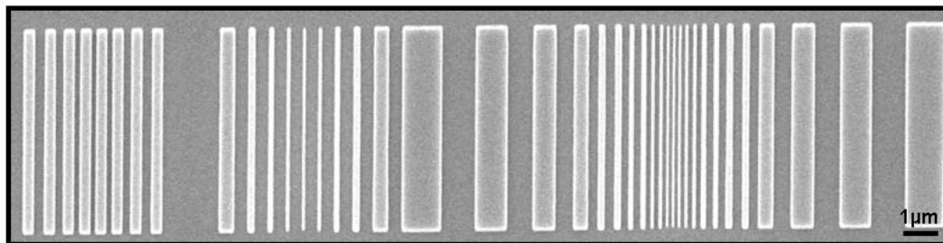
Figure A.4: SEM image (10 kV) of PMMA patterned with the inverted design Fig.B.4. Compared to the PMMA patterns presented in Chapter 4 here the an inverted pattern was written. Nevertheless, the pattern looks well exposed and developed. A sputtered gold film was deposited onto the PMMA for imaging.
