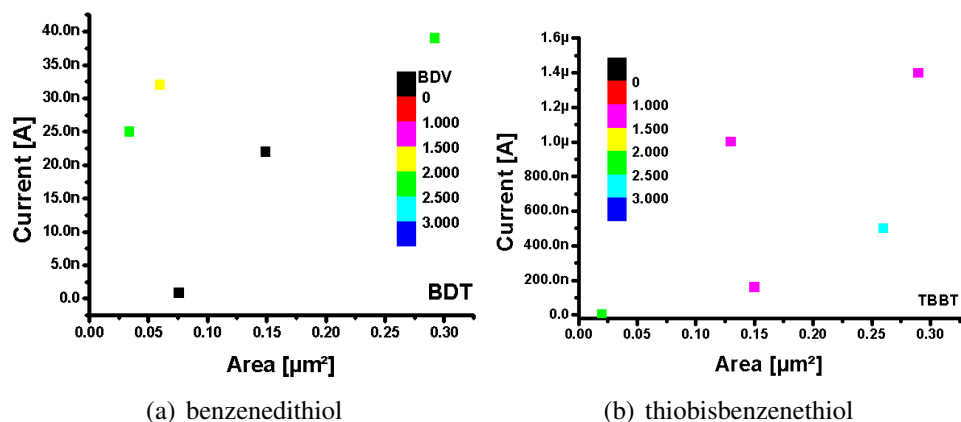
Figure 5.12: Current vs. area plots for conjugated alkanethiols
