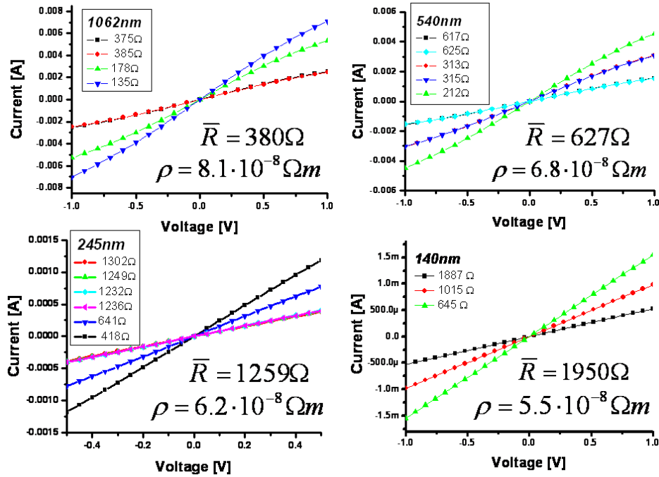
Figure 5.1: Current vs. voltage characteristic for a gold electrodes on Affinity POP 20 nm thick gold electrode with the design shown in Fig.B.8 were transferred onto Affinity VP. The resistance was measured and used to calculate the resistivity.
