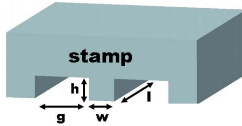
Figure 2.15: Geometry of stamps (for simplicity the pattern consists of parallel lines) h height of the pattern; w width of a line; l length of the pattern lines; g gap between neighboring lines;
