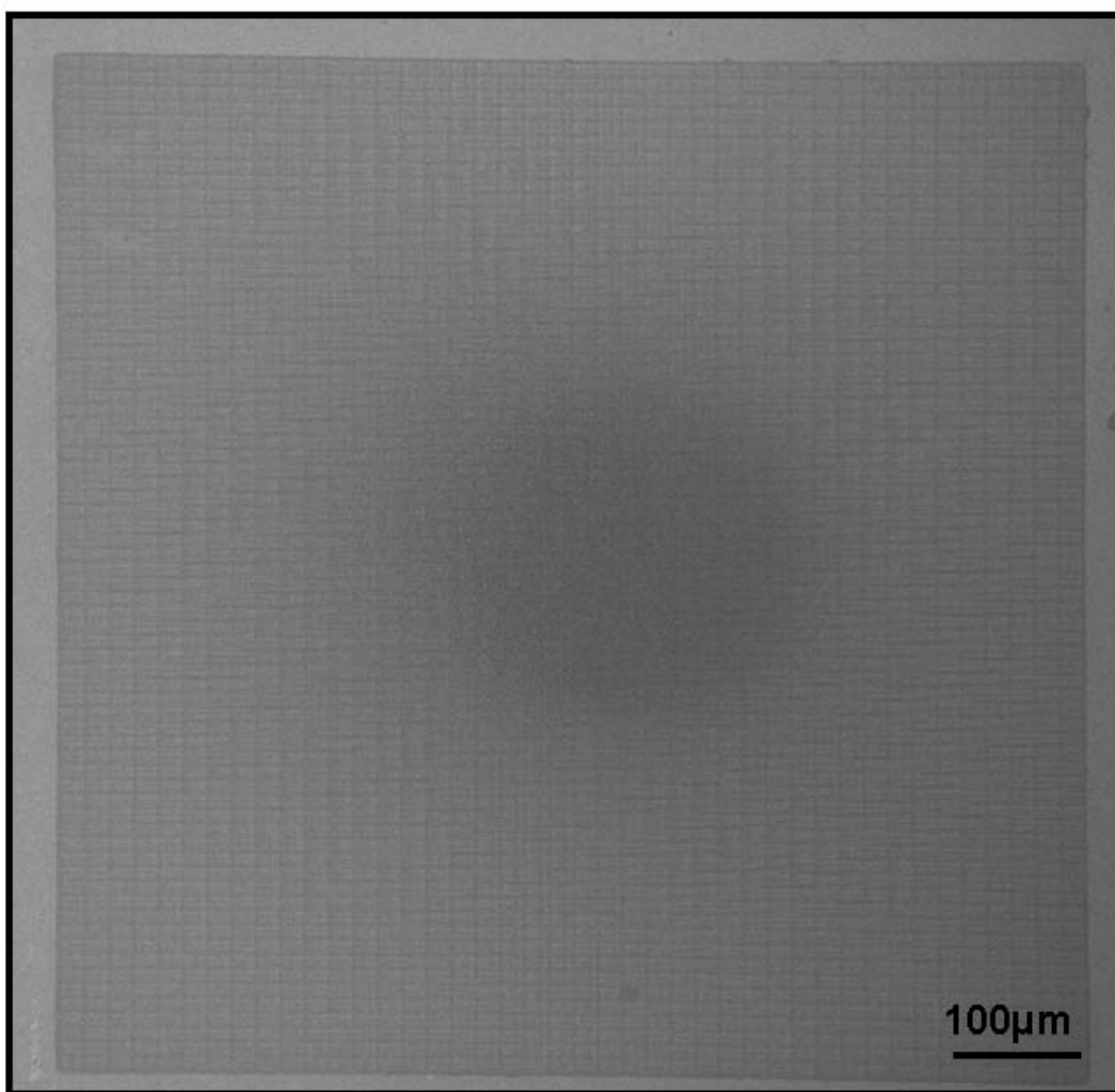
Figure A.17: SEM image (2 kV) of a protein transfer on a 800\ \mu\text{m} \times 800\ \mu\text{m} area Cyt c was printed with Wet Inking and Air-Cushion \mu\text{CP} using a Surlyn stamp having the design shown in Fig.B.4 onto gold. A very homogeneous result was achieved all over the area. Only three defects can be seen.
