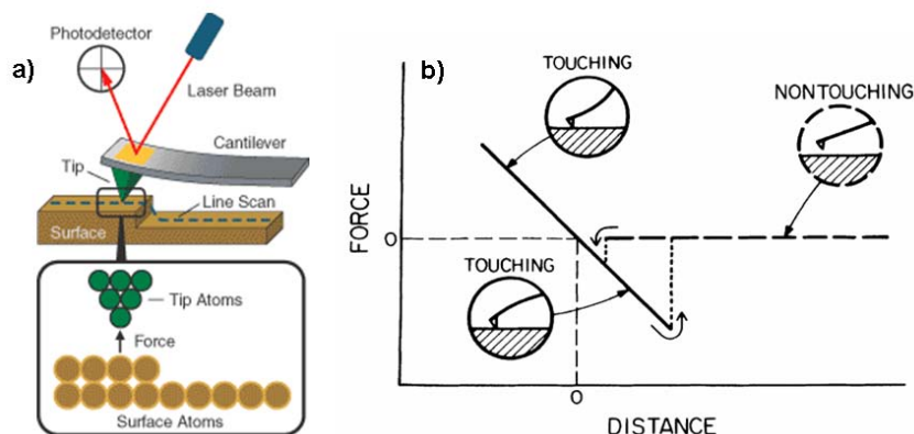
Figure 2.21: Configuration of an AFM;
