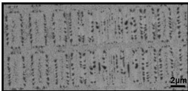
Figure A.8: SEM image (2kV) of residual transfer with Microset PDMS
