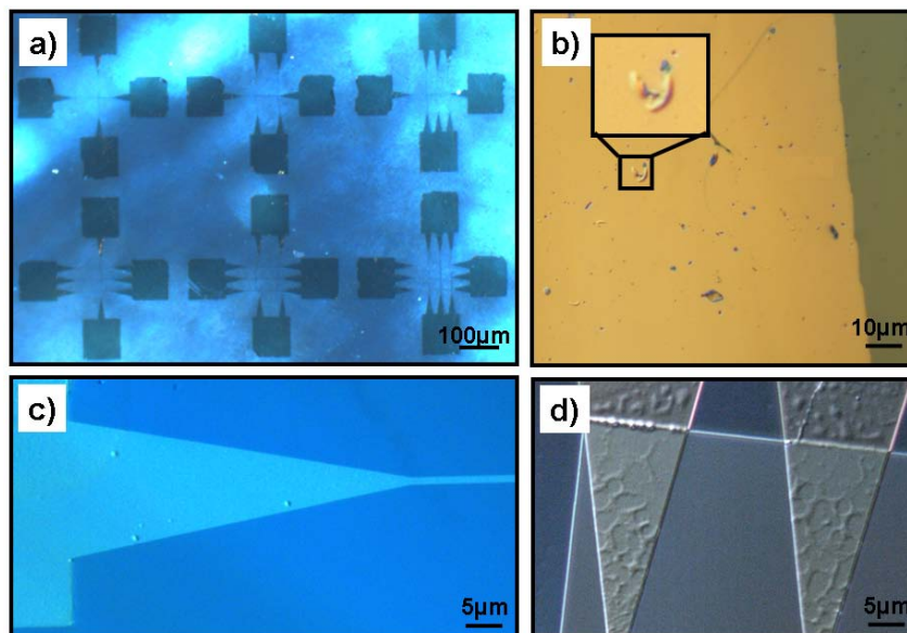
Figure 4.60: Microscope images of transferred gold patterns
