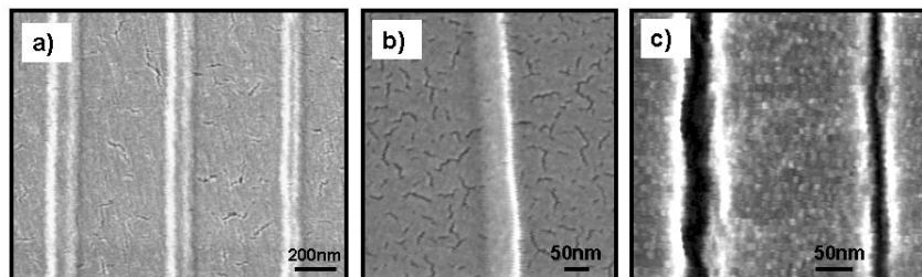
Figure 4.25: SEM images (10 kV) of stamps with sub 75 nm patterns
