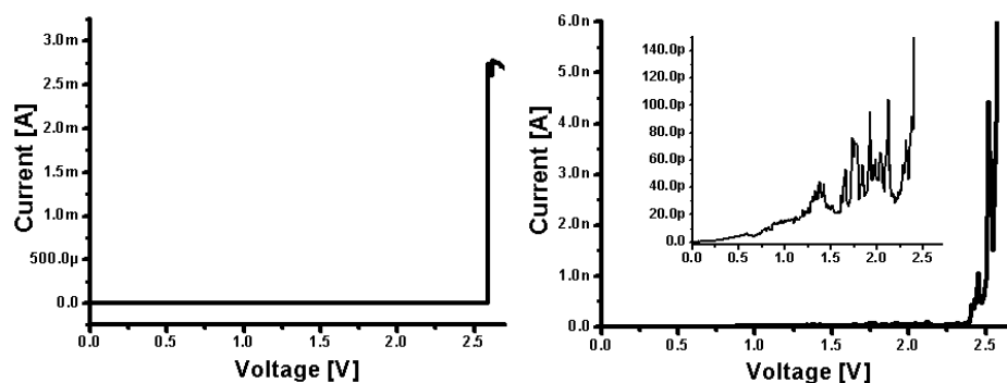
Figure 5.8: Typically break-down characteristic for a alkanethiol junction Hexadecanethiol in a 140 nm by 1 \mu m junction. The right plot is a magnification of the left one. The inset shows even more details.
