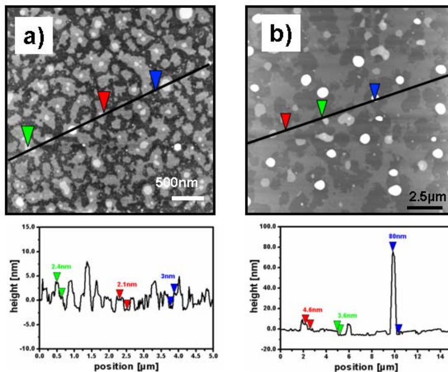
Figure A.6: AFM image of a fluoro-silanized surfaces
