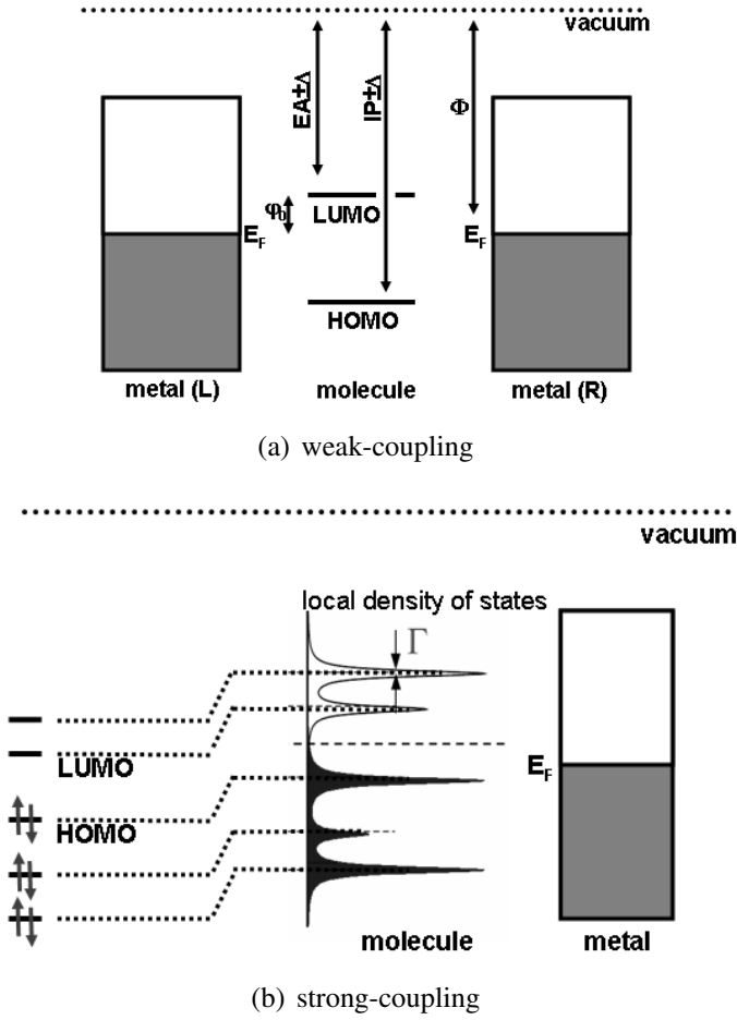
Figure 2.23: Energy plot for a metal/molecule/metal junction in the weak-coupling and strong-coupling approximation; a) adapted from [Lindsay 2005]
