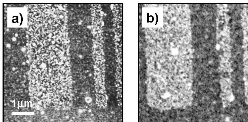
Figure 4.41: Comparison of AFM and SEM images of printed cyt c a 12\ \mu\text{M} cyt c solution in a 0.1\ \text{mM} buffer was printed onto MUA covered gold with a Surlyn stamp using Contact Inking and 2 min printing time a) tapping mode AFM image, z-scale (white contrast) 10\ \text{nm} b) SEM image at 2\ \text{kV} (image contrast was inverted)
