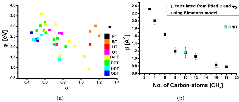
Figure 5.6: Non-short Xbar junctions fitted by Simmons equation
