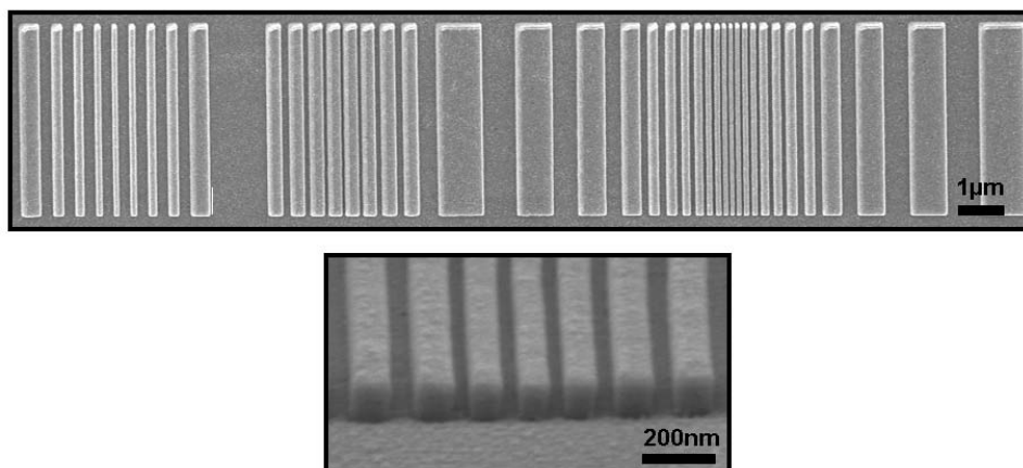
Figure A.9: SEM images (10 kV) of a Topas stamp
