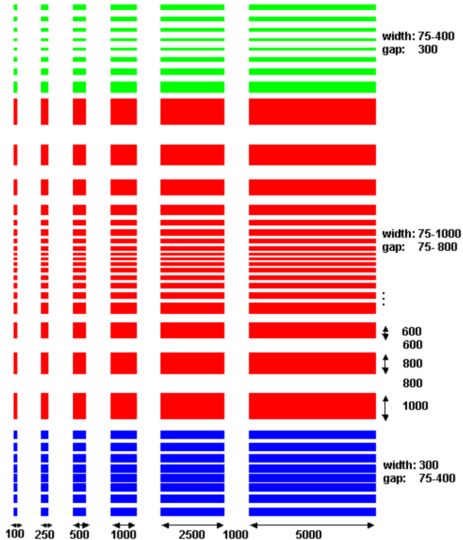
Figure B.4: Design for the 75 nm master
