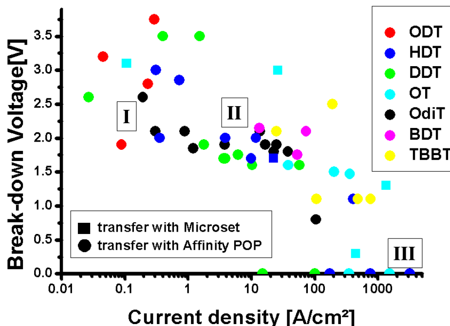
Figure 5.9: Break-down voltage vs. current density for various alkanethiols
