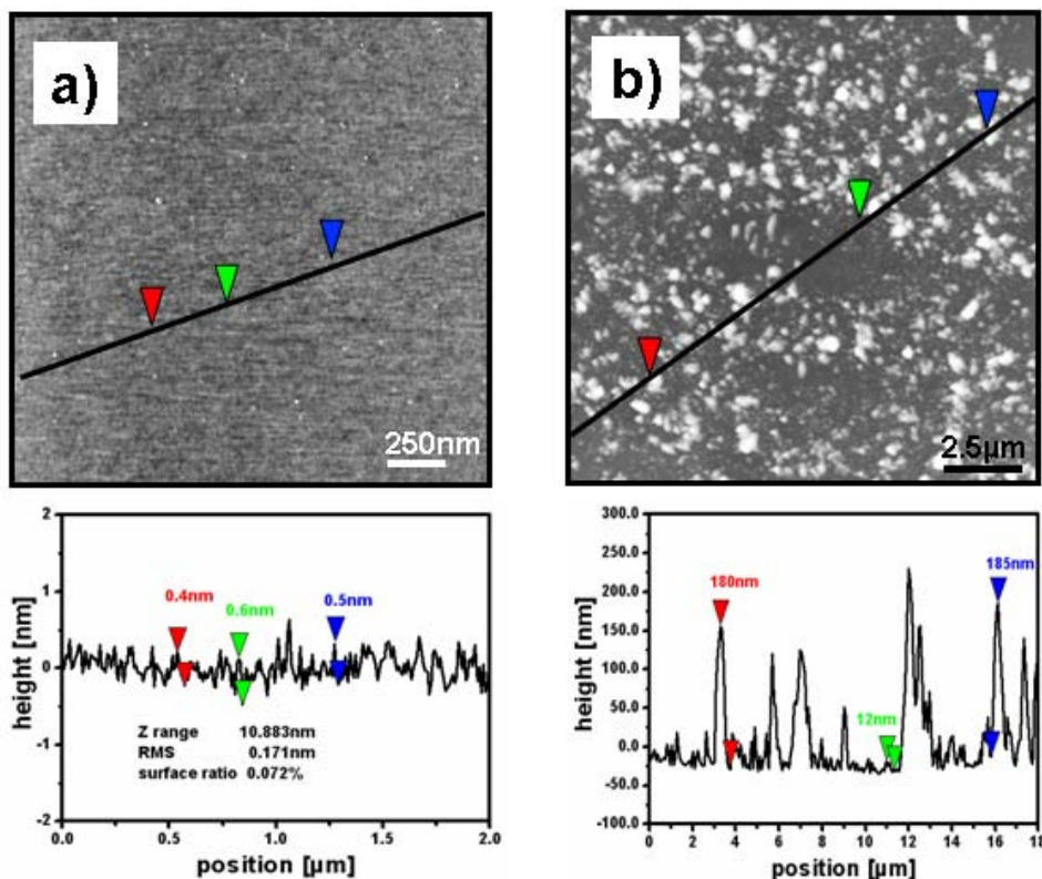
Figure 4.17: AFM image of fluoro-silanized surfaces
