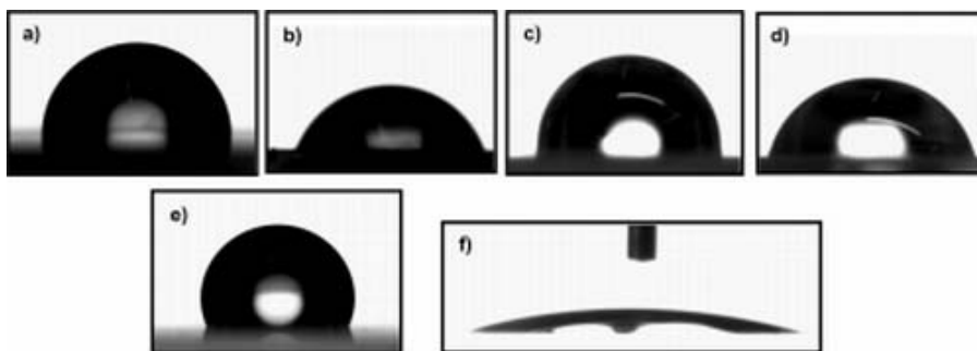
Figure 4.26: Water contact angle of stamp materials
