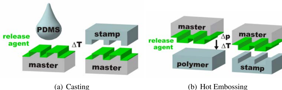
Figure 2.12: Schematics for Casting and Hot Embossing
