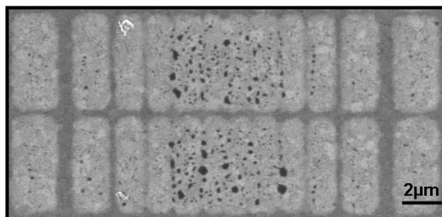
Figure 4.28: SEM image (2 kV) of ODT transferred onto gold with a PDMS stamp
