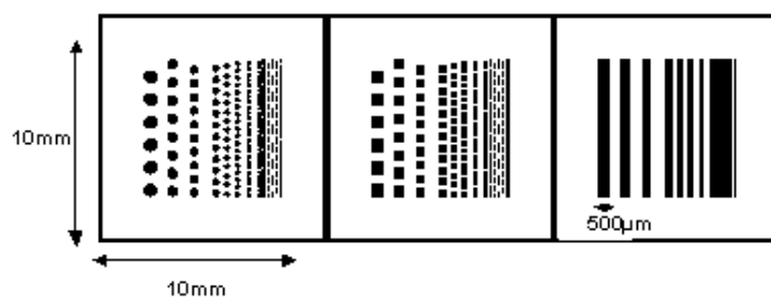
Figure B.1: Design for micron masters with squares, dots and lines ranging between 5\text{ }\mu\text{m} and 500\text{ }\mu\text{m} . This design is realized on a mask for Optical Lithography .
