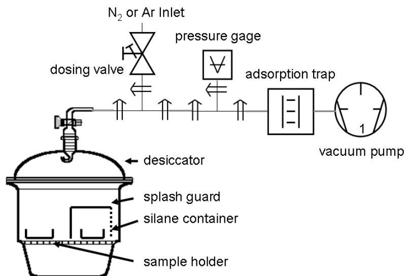
Figure 4.15: Vapor deposition setup for the silanization
