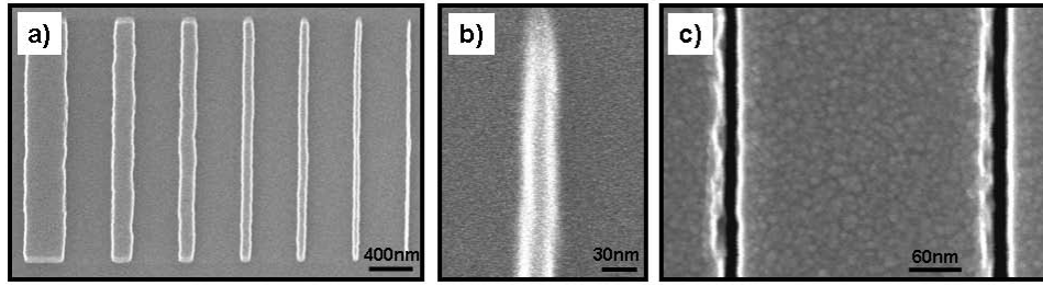
Figure 4.13: Master having sub 50 nm patterns
