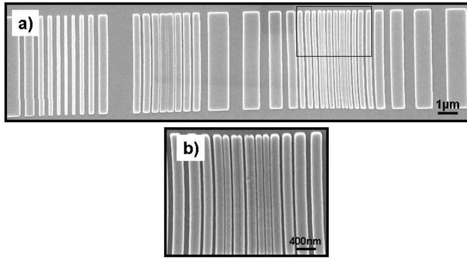
Figure 4.20: Pairing observed for a h-PDMS stamp SEM image (10 kV) of a h-PDMS stamp with a depth of 100 nm and the design shown in Fig.B.4. The stamp was coated with a sputtered gold layer for imaging. b) magnification of the highlighted area
