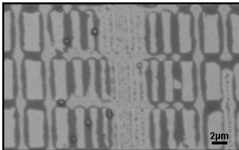
Figure 4.36: SEM image (2 kV) of ECM gel printed with Wet Inking . Extra cellular matrix gel (bright contrast) was printed onto a silicon substrate (dark contrast) with a PDMS stamp (design Fig.B.3). A typical sagging pattern can be seen.
