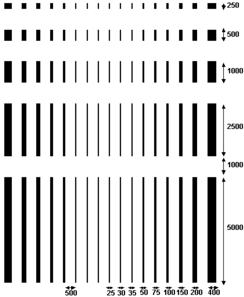
Figure B.5: Design for the 25 nm master
