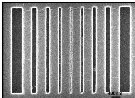
Figure 4.12: Master fabricated under non-perfect conditions SEM image (10 kV) of a PMMA sample patterned with the design shown in Fig.B.4 at 250 \mu\text{C}/\text{cm}^2 , developed using 2 MHz megasonic, etched with a HBr plasma into polysilicon. However, some residues are present in the trenches.
