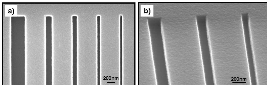
Figure 4.10: Reactive Ion Etching of polysilicon etched through a PMMA mask in several step SEM image (10 kV) of 100 nm polysilicon etched with a HBr plasma using PMMA as an etch mask. The etching was done in a five 30 s steps. a) top-view b) taken under a 70° angle
