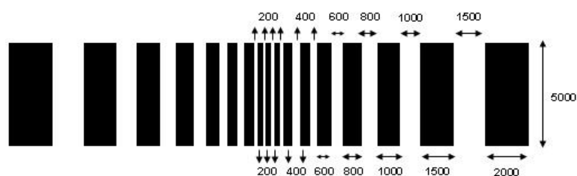
Figure B.3: Design for the 200 nm master
