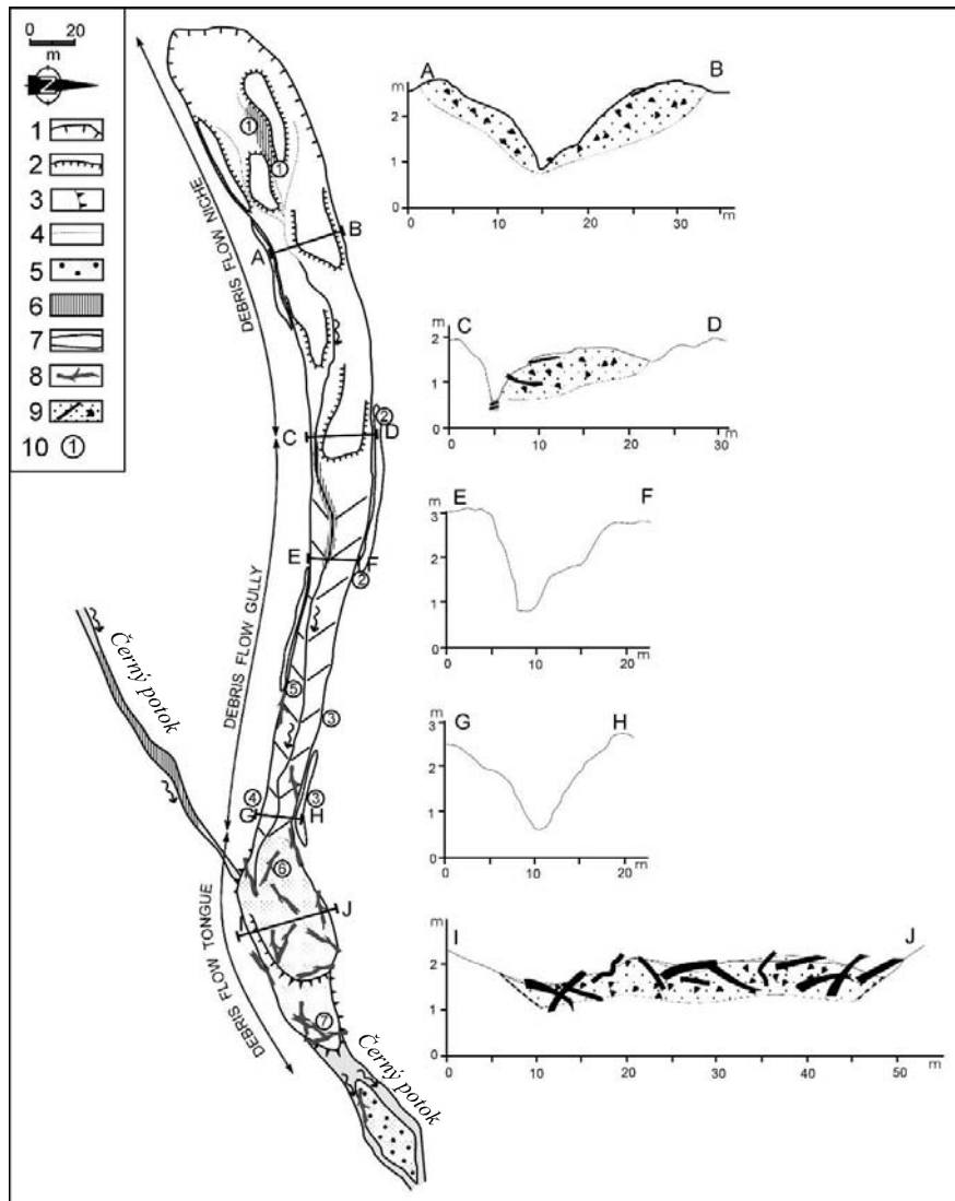
Figure 3: Morphological sketch and cross-section of the debris-flow under study 1 – edge of the niche, 2 – edge of accumulation forms, 3 – debris-flow tongue, 4 – episodically drained small gullies, 5 – depositional river channel forms, 6 – bedrock outcrops, 7 – debris-flow levee, 8 – coarse woody debris, 9 – coarse grained sediments with logs 10 – location of the dendrochronological research sites.
