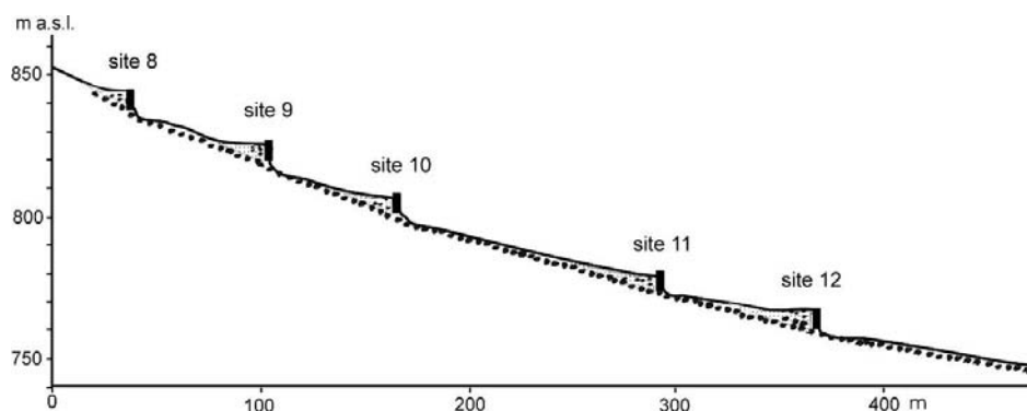
Figure 4: Longitudinal profile of Cerny Potok stream.
