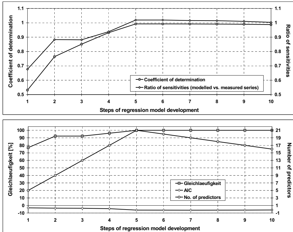
Figure 4: Built up (steps 1 to 5) and backward selection (steps 6 to 10) of the regression model; Number of predictors drops down from 21 to 16. Coefficient of determination, Gleichlaufigkeit and ratio of sensitivities nearly keep their level during backward selection.
