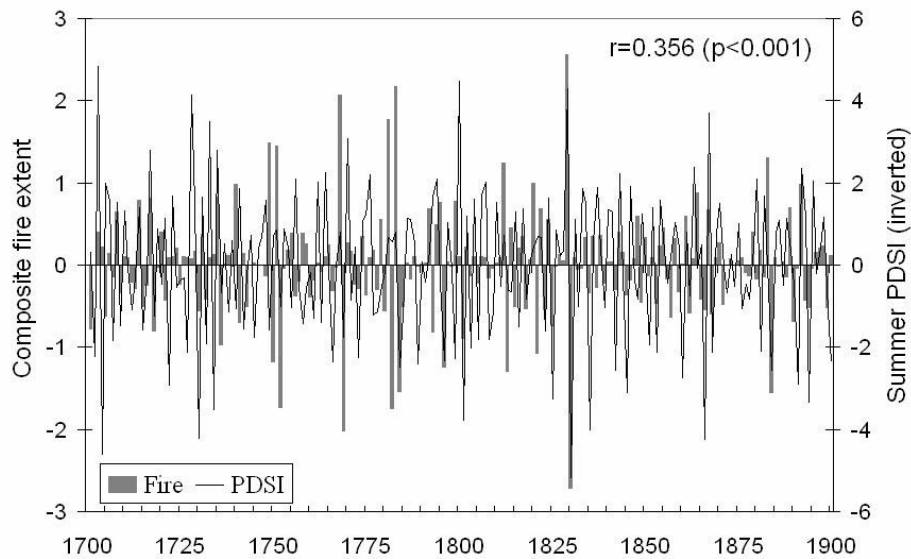
Figure 3: Time series of correlations between a composite time series of fire extent for 7 sites in the southern Cascade Range, California and reconstructed summer PDSI for northern California. PDSI values and corresponding correlation coefficients are inverted to visually enhance the relationship.
