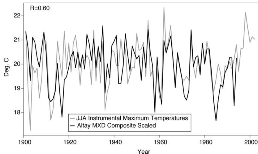
Figure 7: Altay regional composite chronology after scaling to average June-August maximum temperatures.
