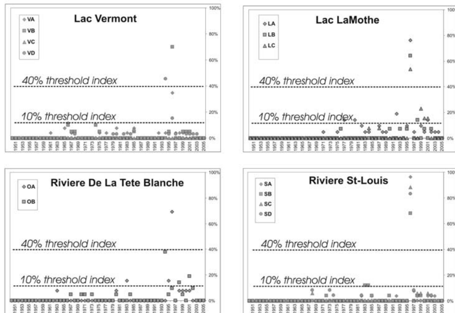
Figure 4: Summarized frequency of scar occurrence for each sampled debris flows at the four investigated sites.
