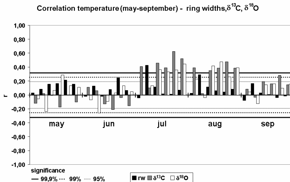
Figure 4: Correlation between ring width, \delta^{13}\text{C} and \delta^{18}\text{O} and temperature during the growth period.
