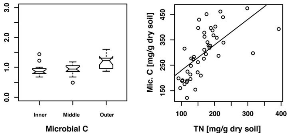
Figure 3: Notched boxplot (left) of microbial C from the inner to the outer zone of influence (standardized on the plot). N=16 . Microbial C is linearly related ( p<0.001 ) to total extractable N (right).
