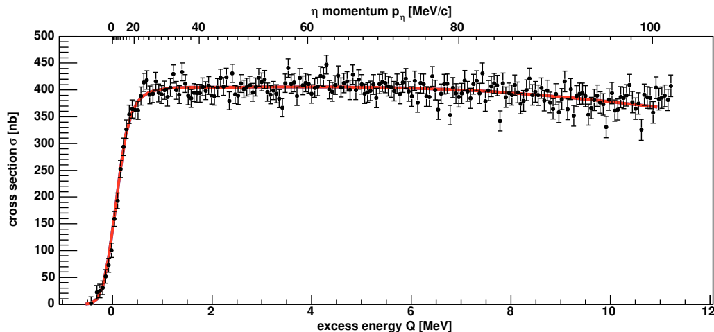
Fig. 1. Total cross section for the dp \rightarrow {}^3\text{He}\eta total cross section measured at COSY-ANKE [1] in terms of the excess energy Q and \eta c.m. momentum p_\eta . The fits with and without the p -waves, as discussed in the text, are indistinguishable and so they are not presented separately.
