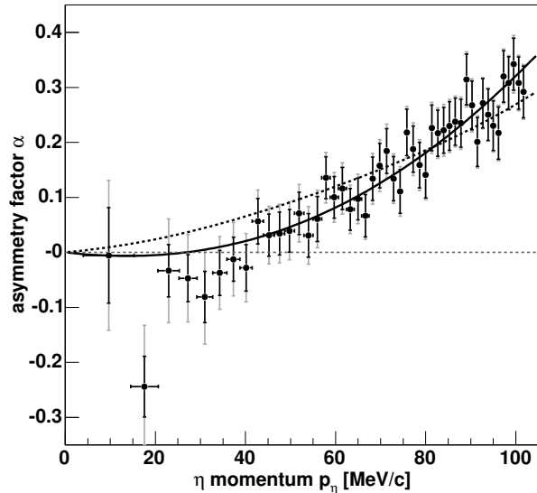
Fig. 2. Variation of the asymmetry parameter \alpha defined by Eq. (1) with the c.m. momentum of the \eta -meson. The solid line is the result of fitting the ANKE data of Ref. [1] with Eq. (8), where the s -wave amplitude f_s of Eq. (6) was introduced. The dashed line was obtained after neglecting the phase variation of f_s , i.e. letting f_s \rightarrow |f_s| . In all cases the fits were carried out by considering only the statistical errors shown by dark lines. Combining these quadratically with the systematic uncertainties leads to the total errors, which are represented by the grey lines.
