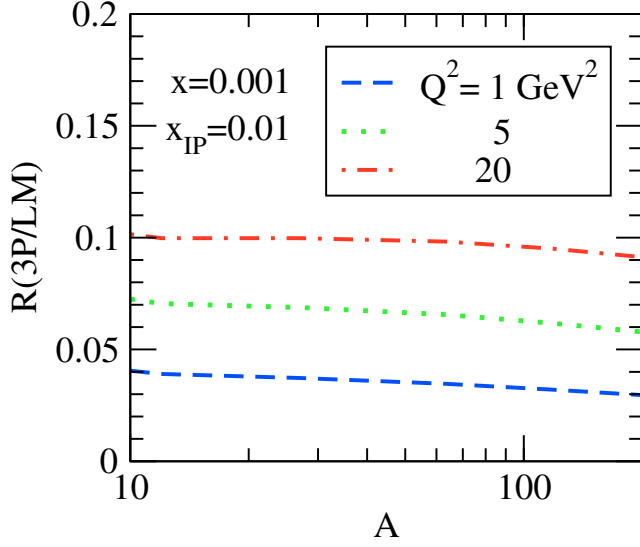
Figure 4: The predicted nuclear mass-number dependence of the ratio, R(3\mathbf{P}/LM) , of the high-mass to low-mass diffractive DIS at several values of Q^2 .
