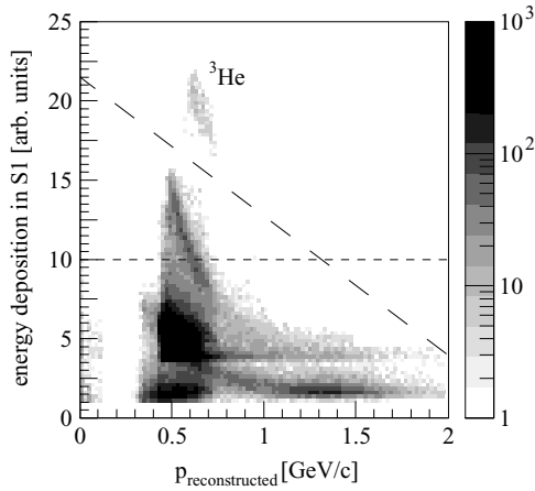
FIG. 2. ^3\text{He} selection from events triggered by the detection system for a beam momentum of 1.593 GeV/c ( Q = 10.8 MeV). Because of the high-energy deposition of the ^3\text{He} nuclei in the scintillator detector S1, ^3\text{He} events can be separated easily from the background consisting of pions, protons, deuterons, and tritons. The dashed lines indicate the cuts on energy loss and the correlation of energy loss to the reconstructed momentum used to select the ^3\text{He} events.
