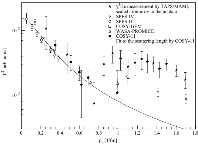
FIG. 9. Squared absolute production amplitude for the \eta - {}^3\text{He} final state in \gamma - {}^3\text{He} and pd collision. The photoproduction data (stars) have been scaled arbitrarily to fit the pd data at p_\eta < 0.8 fm ^{-1} .
