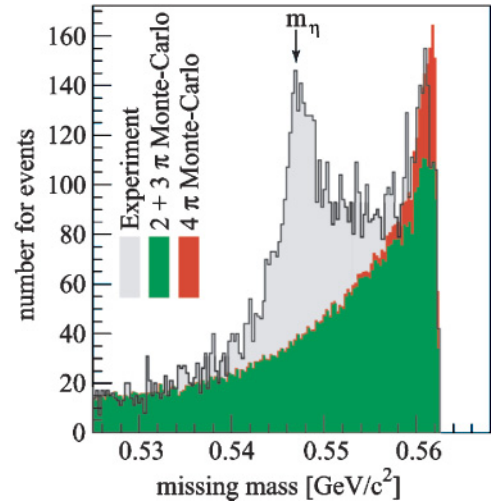
FIG. 3. (Color online) Missing-mass distribution obtained for ^3\text{He} events, recorded at an excess energy of 15.1 MeV. On top of the background, a peak in the range of the \eta mass ( m_\eta = 0.5473 GeV/c 2 ) is quite prominent. By combining Monte Carlo events from reactions of the type pd \rightarrow ^3\text{He}n \cdot \pi (n \geq 2) the background observed in the experiment can be described very well. The simulation was fit in magnitude to the experimental data in the region outside the \eta signal; for details see text.
