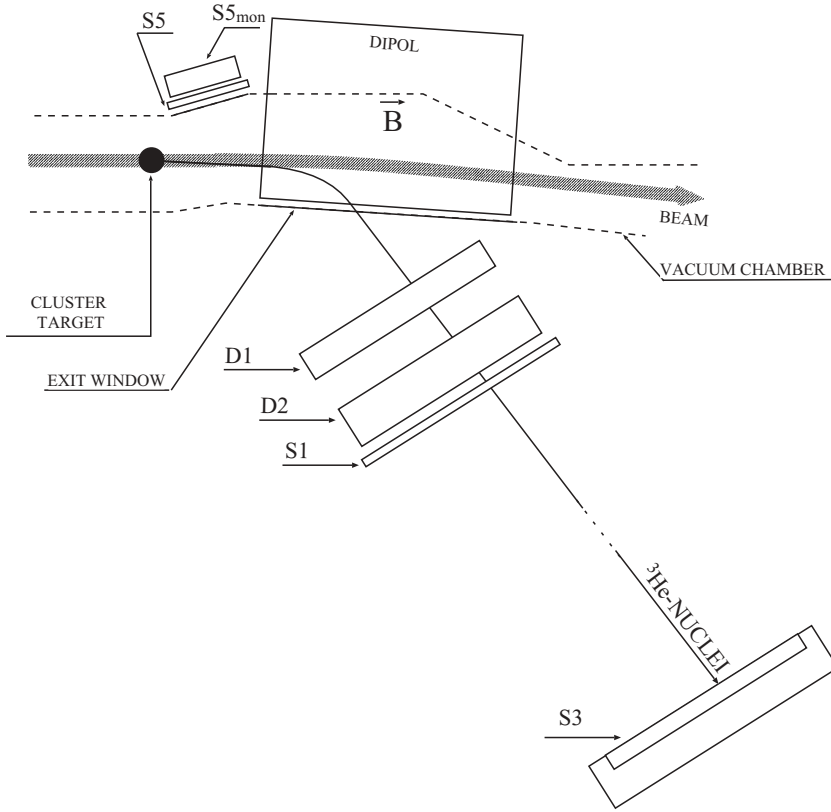
FIG. 1. Sketch of COSY-11 installation. The magnetic spectrometer, consisting of drift chambers and scintillation and silicon-pad detectors is located in an arc region of the cooler synchrotron COSY at the Forschungszentrum Jülich.
