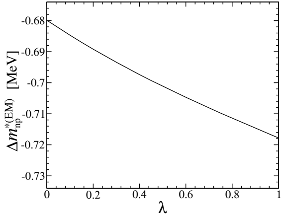
Fig. 2. Density dependence of the electromagnetic part of the neutron-proton mass difference. The abscissa represents \lambda = \rho/\rho_0 , while the ordinate represents \Delta m_{np}^{*(EM)} in units of MeV.
