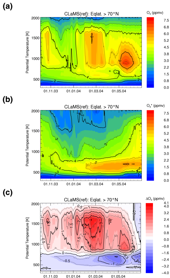
Fig. 2. Mean distributions, poleward of 70° N equivalent latitude, of (a) ozone, (b) passively transported ozone (O 3 * ), and (c) the accumulated chemical ozone change (ΔO 3 =O 3 −O 3 * ) from the reference simulation performed with CLaMS.
