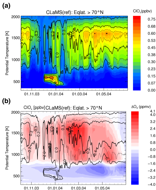
Fig. 4. (a) Time series of the mean distribution of activated chlorine ( \text{ClO}_x = \text{ClO} + 2 \times \text{Cl}_2\text{O}_2 ) poleward of 70° equivalent latitude for the reference model run. Panel (b) shows the chemical ozone change same as Fig. 2c, but with contour lines of the mean distribution of \text{ClO}_x . It is clearly shown that the region of chlorine activation caused by PSC occurrence is mainly in the lower part of the region where most ozone loss occurred at that time.
