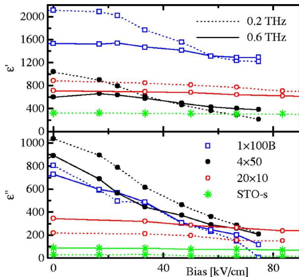
FIG. 3. (Color online) Real and imaginary parts of the dielectric function of STO films as a function of external electric field.
