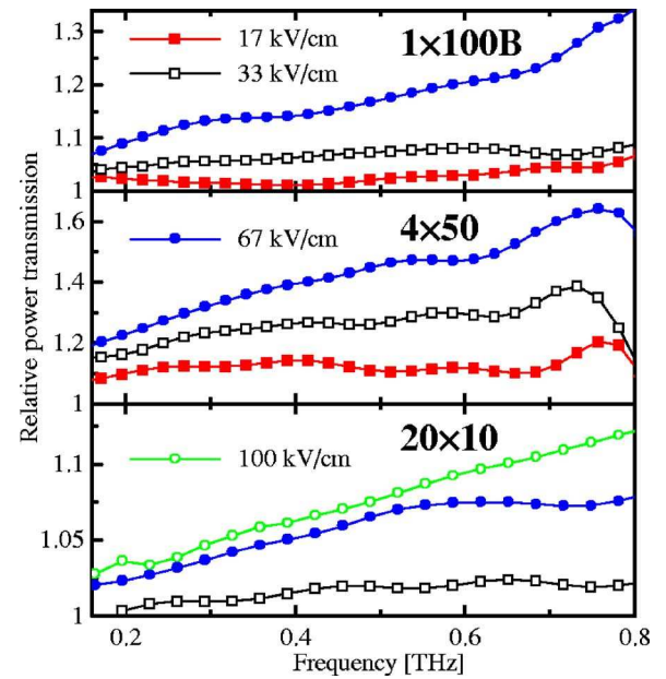
FIG. 2. (Color online) Power transmission spectra of the investigated samples. We plot here the ratio between the terahertz transmittances with and without bias: |E_V/E_0|^2 .
