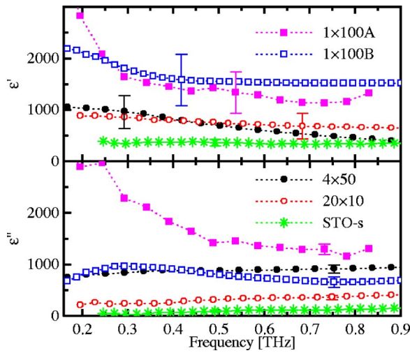
FIG. 1. (Color online) Zero-field permittivity and losses of STO films.
