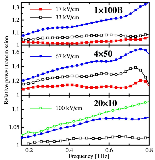
FIG. 2. (Color online) Power transmission spectra of the investigated samples. We plot here the ratio between the terahertz transmittances with and without bias: |E_V/E_0|^2 .
