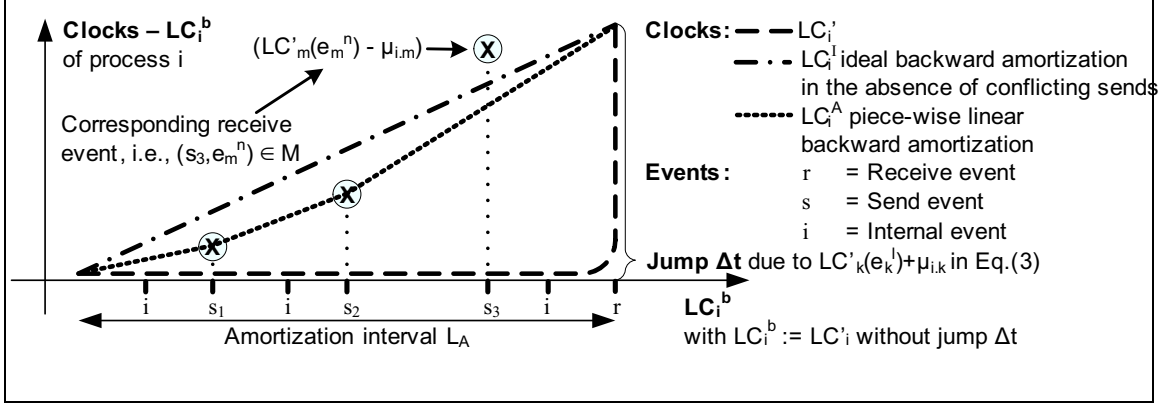
Figure 3.1: Algorithm for backward amortization.
