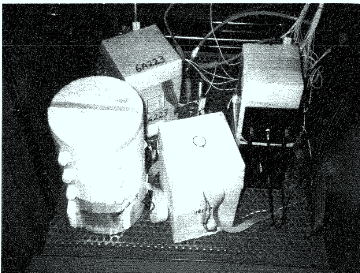
Figure 13: Four different ozone sondes installed in the environmental simulation chamber just prior to a simulation of an ozone sounding during JOSIE-1996
