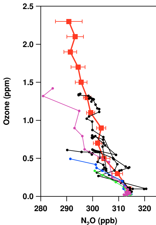
Fig. 11. Scatterplot of ozone vs \text{N}_2\text{O} . Solid red squares represent the averages of non-Davina profiles (in bins of 0.1 ppm ozone) observed during the campaign, with range bars showing \pm 1 standard deviation. Black circles connected by lines are the profiles from a sub-sample of the campaign dataset with observations southward of 13^\circ \text{S} , (not comprising the Davina flight). Blue, green and purple circles connected by lines denote the profiles obtained respectively on portions A, B and C during the Davina flight.
