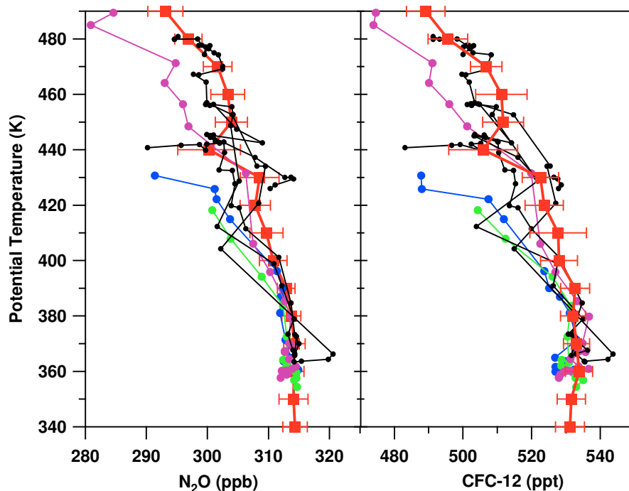
Fig. 8. Mixing ratios of N 2 O (left panel) and CFC-12 (right panel) measured by HAGAR vs potential temperature. Red squares represent the averages of non-Davina profiles (in 10 K bins of potential temperature) observed during the campaign, with range bars showing \pm 1 standard deviation. Black circles connected by lines are the profiles from a sub-sample of the campaign dataset with observations southward of 13° S, (not comprising the Davina flight). Blue, green and purple circles connected by lines denote the profiles obtained respectively on portions A, B and C during the Davina flight.
