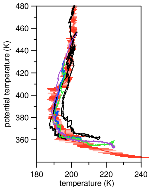
Fig. 5. Temperature vs potential temperature. Solid red lines represent the average non-Davina profiles observed during the campaign, range bars show \pm 1 standard deviation. Black lines are the profile from a subsample of the campaign dataset with observations southward of 13^\circ S, (not comprising the Davina flight). Blue, green and purple profiles denotes the profiles obtained respectively on portions A, B and C during the Davina flight.
