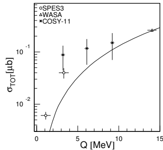
Fig. 3. Dependence of total cross section on the excess energy. The line indicates three body phase-space normalized to the PROMICE/WASA point 11 . Open circles shows data from reference 9 , and stars denotes preliminary results determined by the COSY-11 group.
