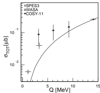
Fig. 3. Dependence of total cross section on the excess energy. The line indicates three body phase-space normalized to the PROMICE/WASA point 11 . Open circles shows data from reference 9 , and stars denotes preliminary results determined by the COSY-11 group.
