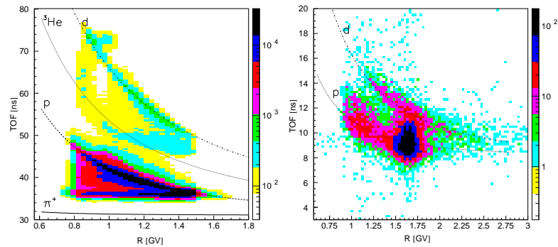
Fig. 2. Dependence of the TOF on magnetic rigidity for particles registered in the drift chambers D1, D2 (left panel) and for particles detected in the D4 chamber (right panel).
