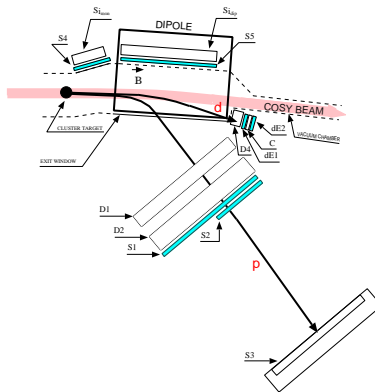
Fig. 1. Detection setup of the COSY-11 experiment 18 . Protons from the dp \rightarrow dp\eta reaction are measured in the drift chambers D1, D2, as well as in the scintillator hodoscopes S1, S3. For detection of the outgoing deuterons, small drift chamber D4 with hexagonal cells 19 , two scintillator detectors dE1, dE2 and Cerenkov threshold counter were installed.
