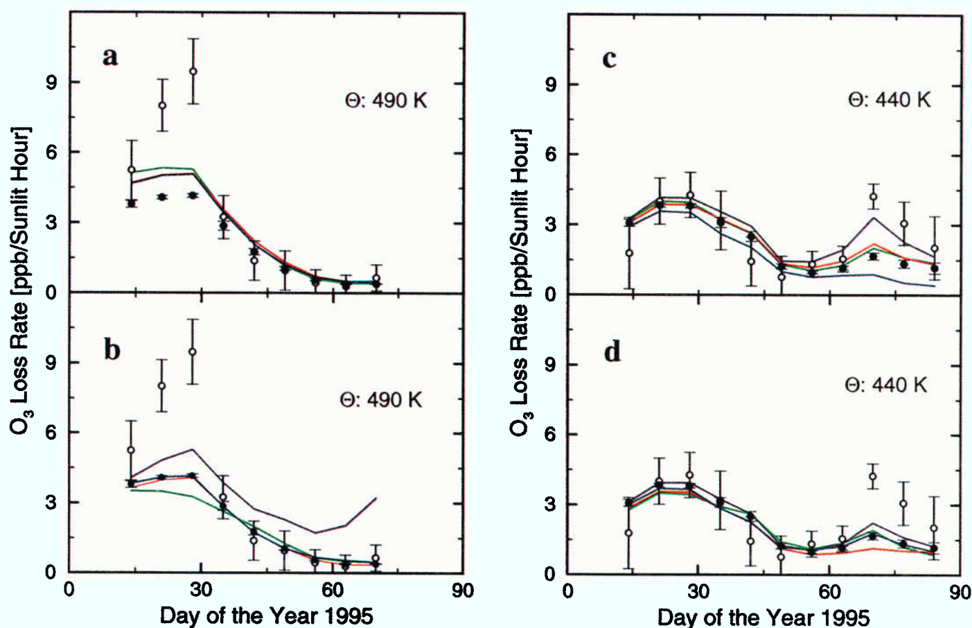
Plate 3. Sensitivity studies. The solid circles correspond the reference case, and the open circles correspond to the Match results. (a) Results for 490 K: Simulations with doubled Cl 2 O 2 photolysis rate and Cl 2 O 2 formation rate constant chosen as the upper limit of the uncertainties according to DeMore et al. [1997] (green line), simulations with doubled BrCl photolysis rate and rate constants of the reactions ClO + BrO → BrCl + O 2 / Br + ClOO chosen as the upper limit of the uncertainties according to DeMore et al. [1997] (red line), simulations with O 3 photolysis rate doubled and rate constant of the reaction ClO + O → Cl + O 2 chosen as the upper limit of the uncertainties according to DeMore et al. [1997] (blue line). (b) Further results for 490 K: Simulations along Match trajectories expanded an additional 10 days backward (green line), along Match trajectories without temperature correction (red line), with short-term temperature fluctuations of 10 K instead of a constant temperature correction (blue line), and simulations without chlorine deactivating reactions (violet line). (c) Results for 440 K: with an additional reaction channel HO 2 + ClO → HCl + O 3 [ Finkbeiner et al. , 1995] with a 3% branching ratio (green line), with doubled background aerosol surface area (red line), with dehydration to ≈ 3 ppm H 2 O (blue line), and with a combination of the reaction channel HO 2 + ClO → HCl + O 3 , dehydration and a temperature reduction of 3 K (violet line). (d) Further results for 440 K: like Plate 3b, except simulations along Match trajectories with a temperature correction of -3 K (violet line).
